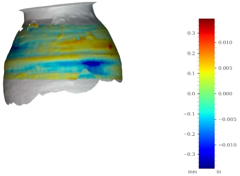
Figure 59: Surface variability heatmap of MV004c, rotated 180°
