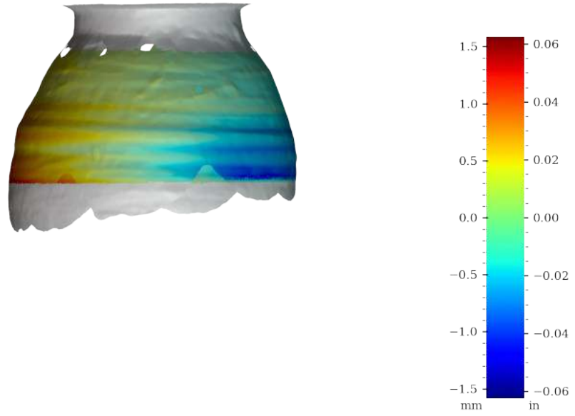
Figure 55: Surface variability heatmap of MV004c, rotated 180°
