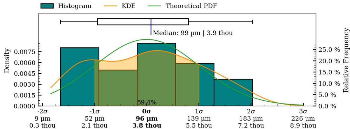
Figure 48: Coaxiality residual plots of interior_separate surface, MV004c.
