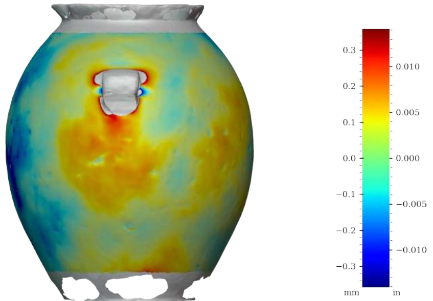
Figure 52: Surface variability heatmap of MV004c, rotated 270°
