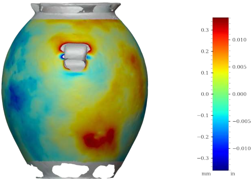
Figure 50: Surface variability heatmap of MV004c, rotated 90°
