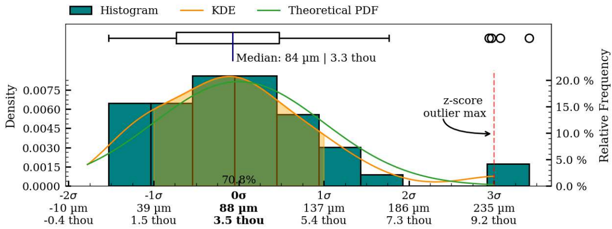
Figure 47: Coaxiality residual plots of interior surface, MV004c.
