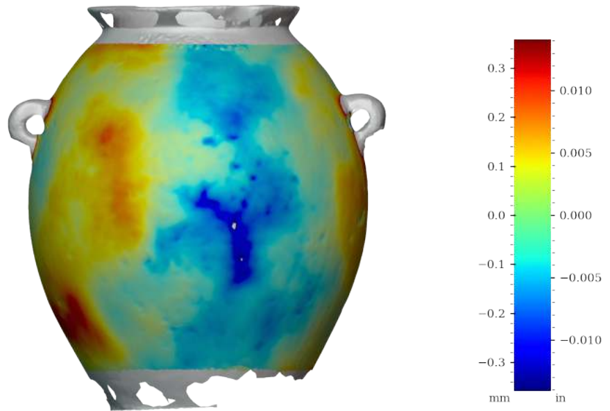
Figure 51: Surface variability heatmap of MV004c, rotated 180°
