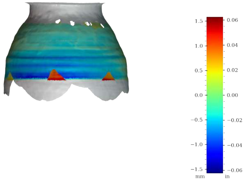
Figure 56: Surface variability heatmap of MV004c, rotated 270°
