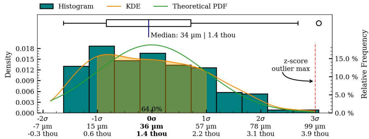
Figure 46: Coaxiality residual plots of exterior surface, MV004c.
