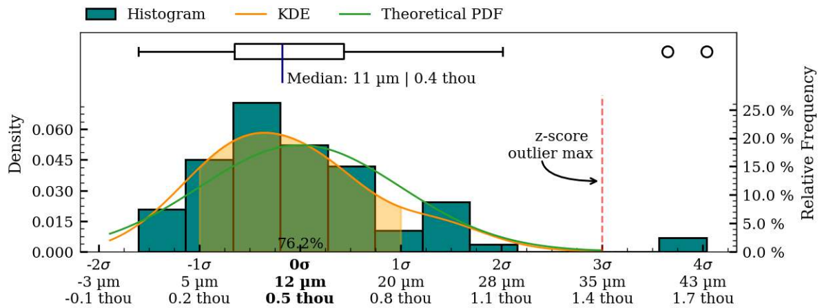
Figure 40: Coaxiality residual plots of interior_separate surface, MV005.
