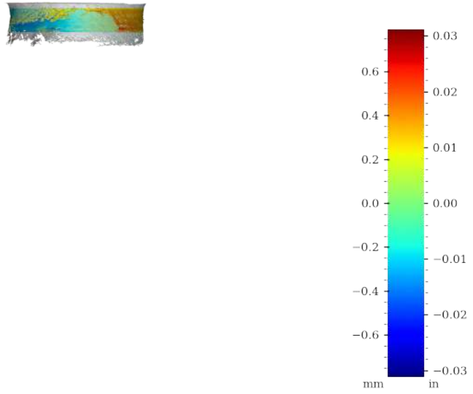
Figure 47: Surface variability heatmap of MV005, rotated 180°
