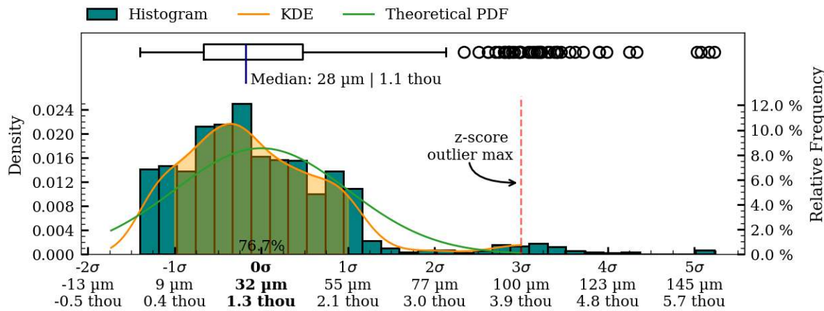
Figure 38: Coaxiality residual plots of exterior surface, MV005.
