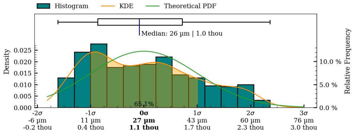
Figure 52: Coaxiality residual plots of interior_separate surface, MV006.
