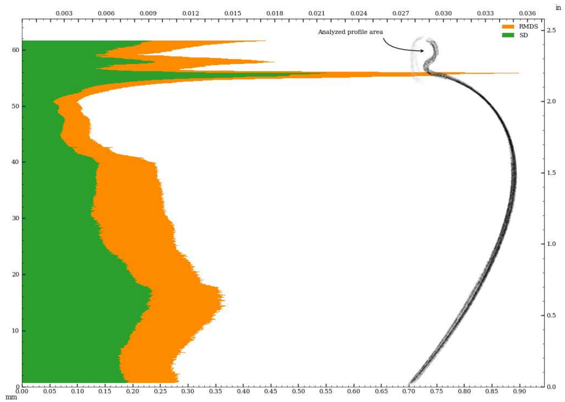
Figure 46: Vessel circularity of exterior surface, in z-plane, standard deviation and median absolute deviation.
