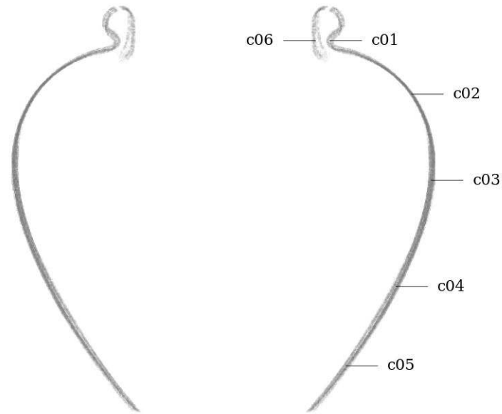
Figure 41: Circularity measurement sample locations, full mesh aligned to exterior surface
