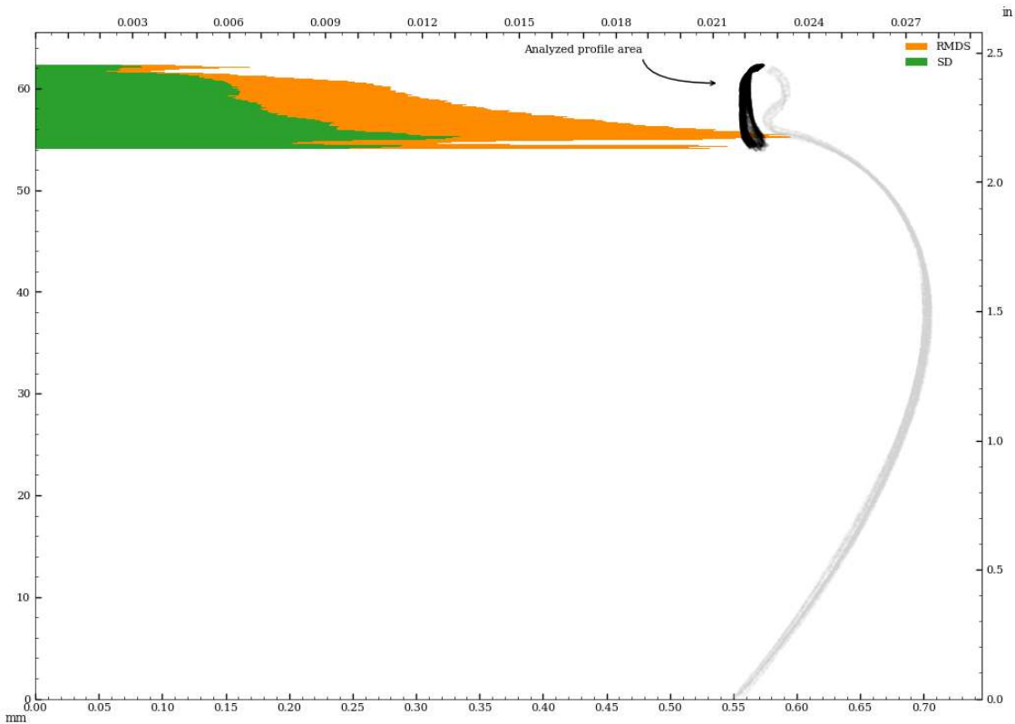
Figure 49: Vessel circularity of interior surface, perpendicular to surface curvature, standard deviation and median absolute deviation.
