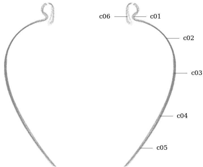
Figure 22: Circularity measurement sample locations, full mesh aligned to exterior surface
