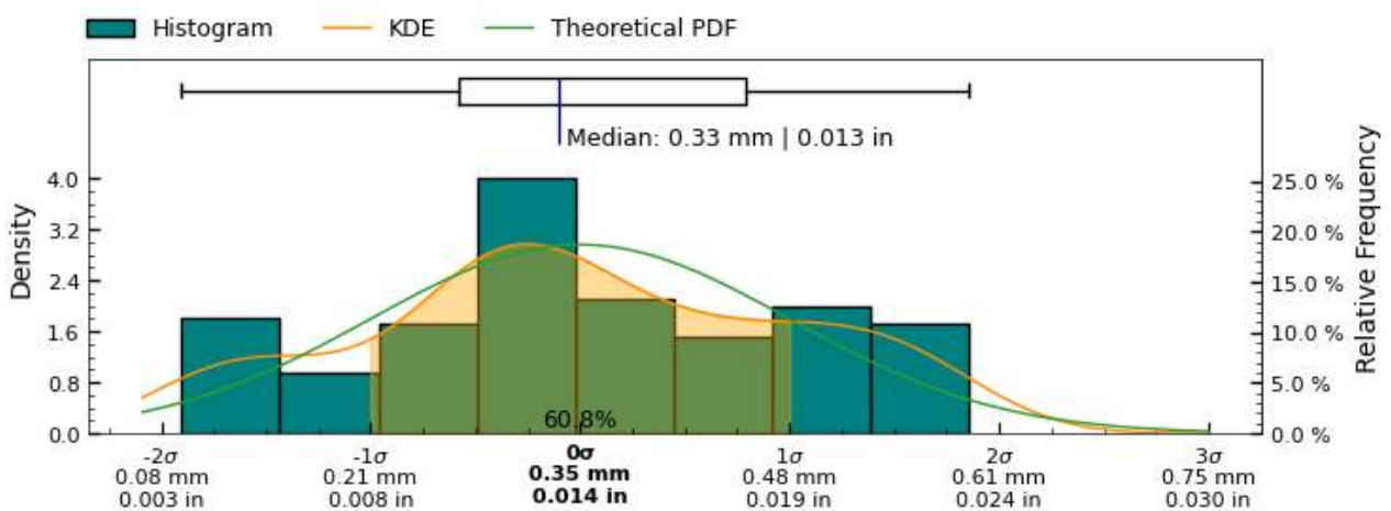
Figure 20: Root Mean Squared Deviation measurement distribution across measured slices of interior surface
