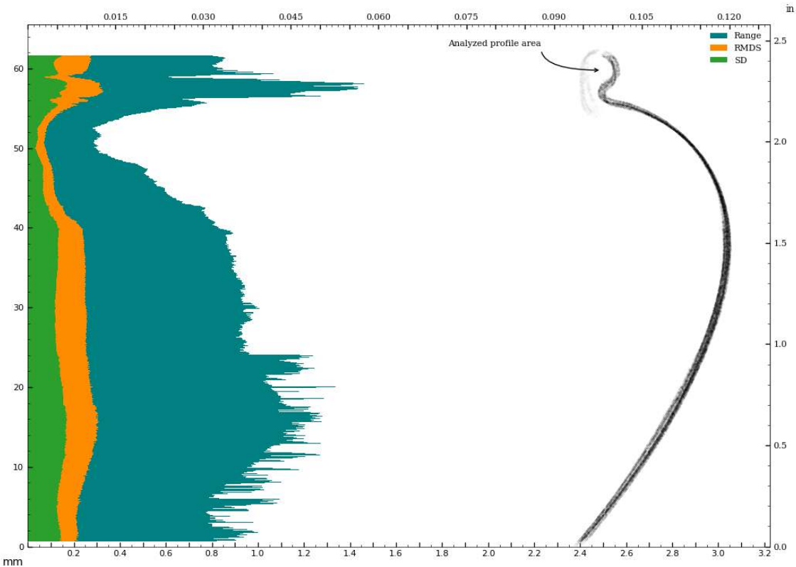
Figure 43: Circularity of exterior surface - perpendicular to surface curvature.
