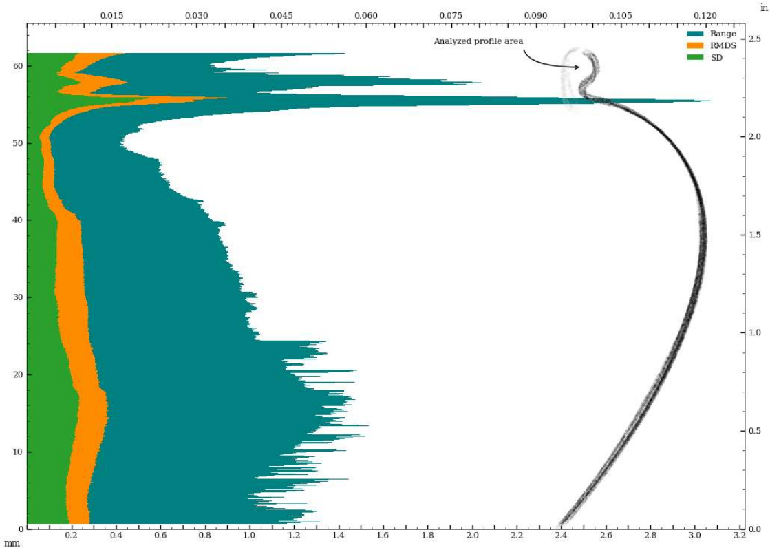
Figure 44: Circularity of exterior surface - in z-plane.
