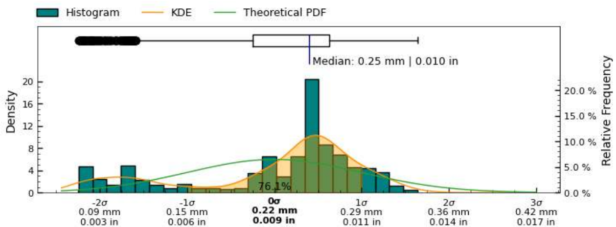
Figure 15: Root Mean Squared Deviation measurement distribution across measured slices of exterior surface
