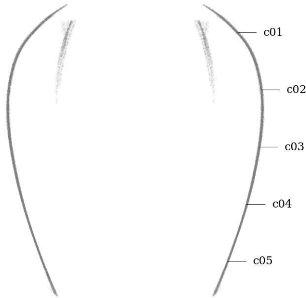
Figure 49: Circularity measurement sample locations, full mesh aligned to exterior surface
