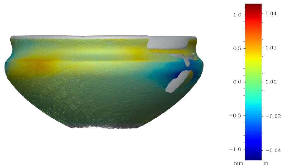
Figure 56: Surface variability heatmap of MV009, rotated 270°
