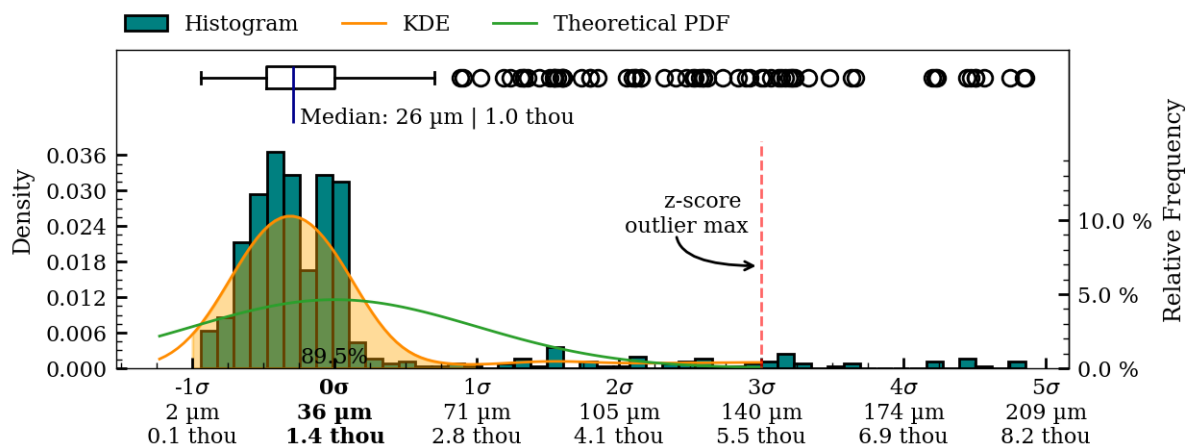
Figure 52: Coaxiality residual plots of interior_separate surface, MV009.
