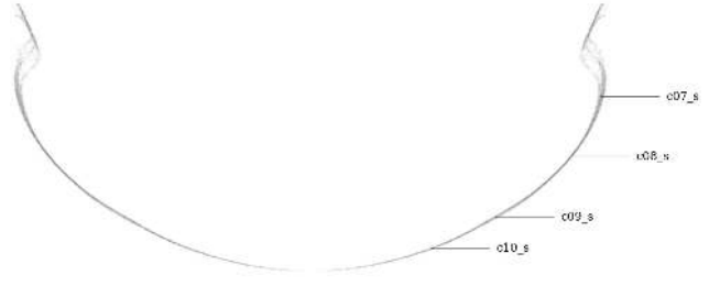
Figure 69: Circularity measurement sample location, separately aligned interior mesh
