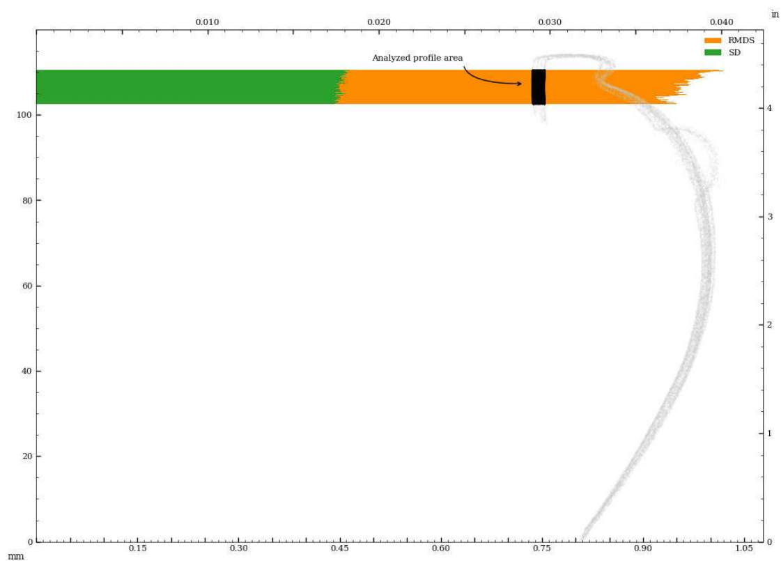
Figure 64: Vessel circularity of interior surface, perpendicular to surface curvature, standard deviation and median absolute deviation.
