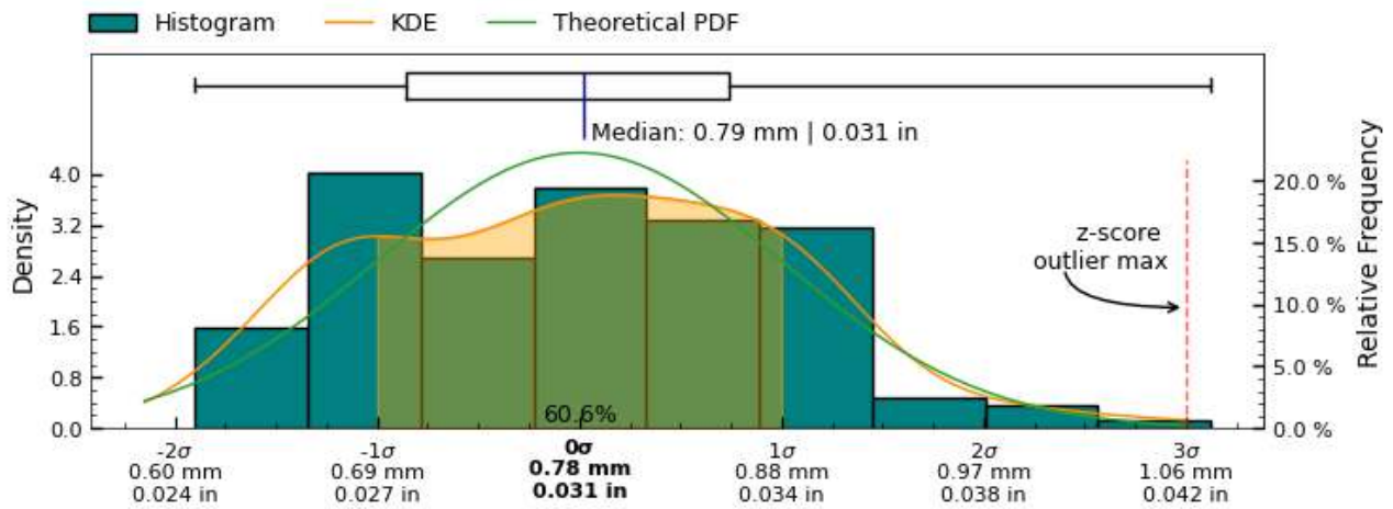
Figure 24: Range measurement distribution across measured slices of interior_separate surface
