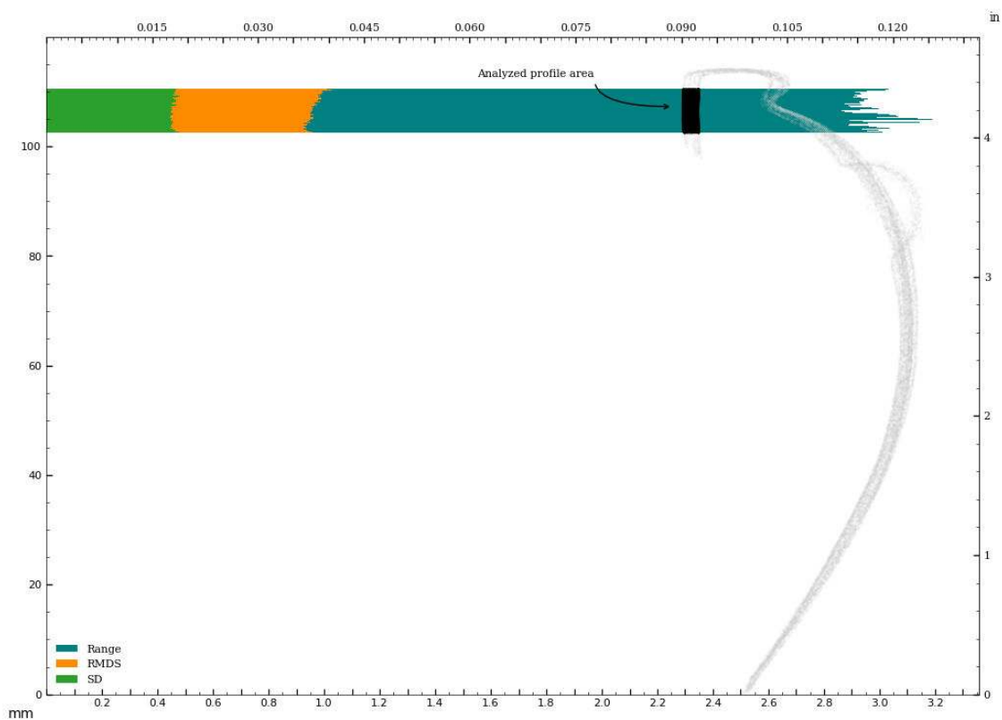
Figure 63: Circularity of interior surface - in z-plane.
