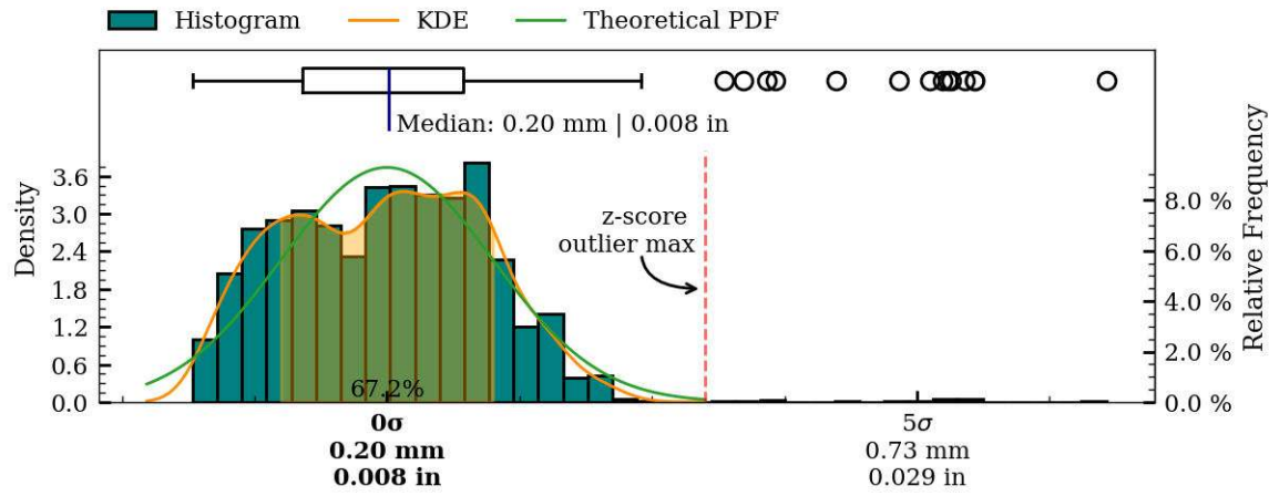
Figure 36: Coaxiality residual plots of exterior surface, MV011.
