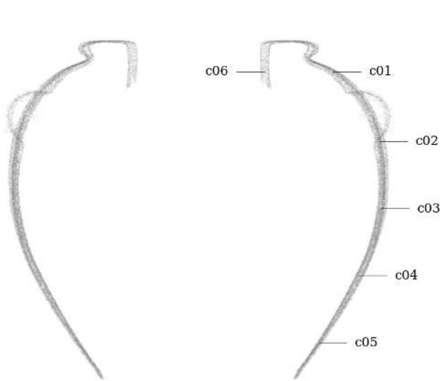
Figure 70: Circularity measurement sample locations, full mesh aligned to exterior surface
