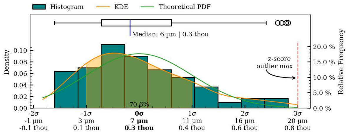
Figure 37: Coaxiality residual plots of interior surface, MV011.
