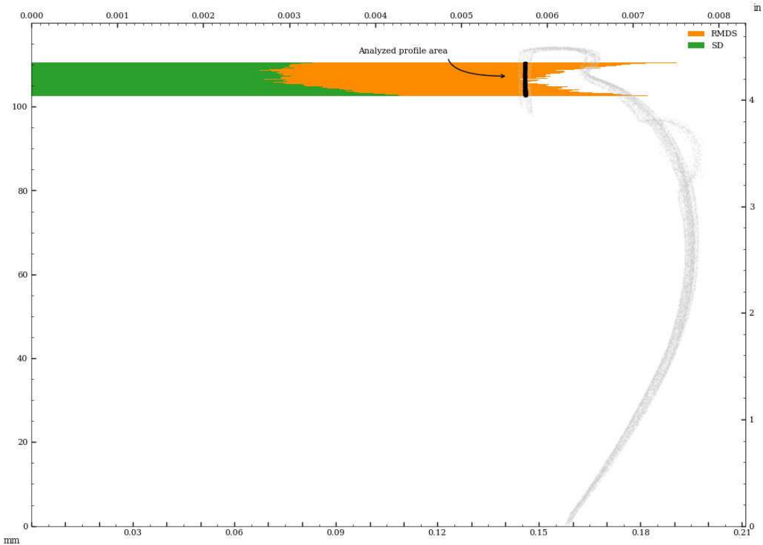
Figure 68: Vessel circularity of interior_separate surface, perpendicular to surface curvature, standard deviation and median absolute deviation.
