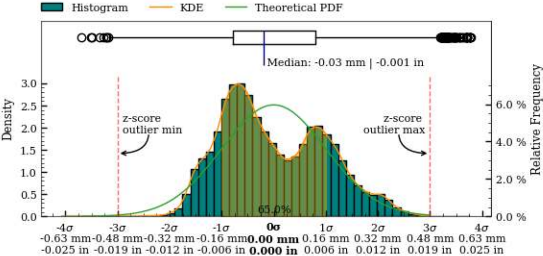
Figure 53: Interior separately aligned surface variability boxplot, kds and histogram.
