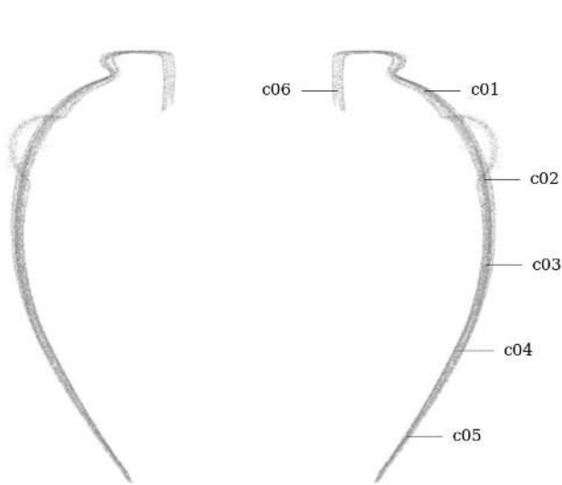
Figure 4: Circularity measurement sample locations, full mesh aligned with exterior surface
