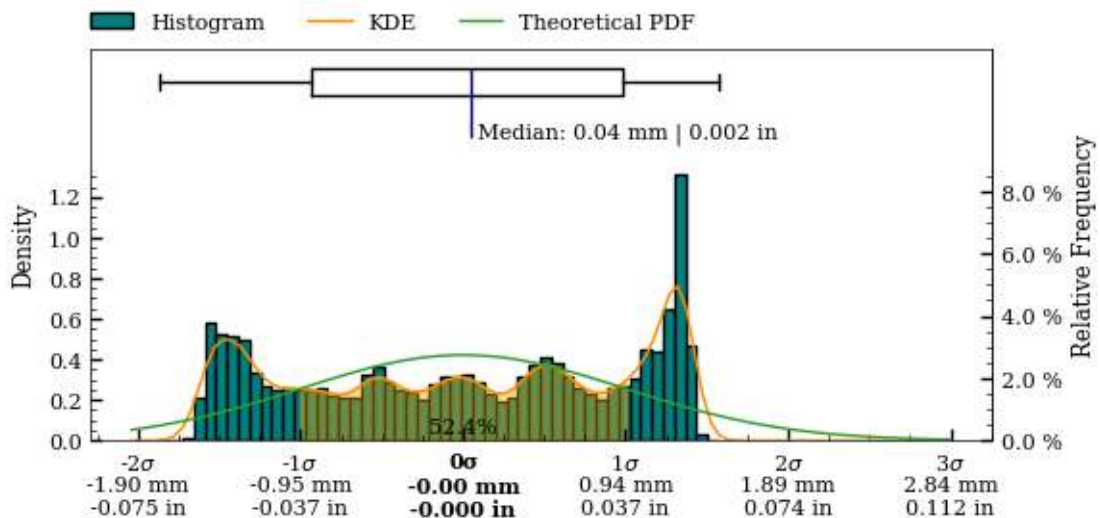
Figure 52: Interior surface variability boxplot, kds and histogram.
