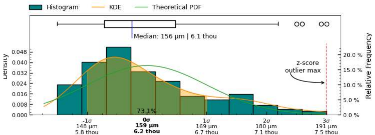
Figure 26: Root Mean Squared Deviation measurement distribution across measured slices of interior separately aligned surface
