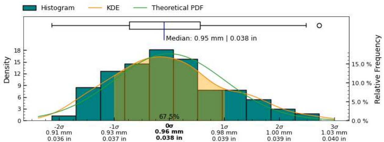
Figure 21: Root Mean Squared Deviation measurement distribution across measured slices of interior surface
