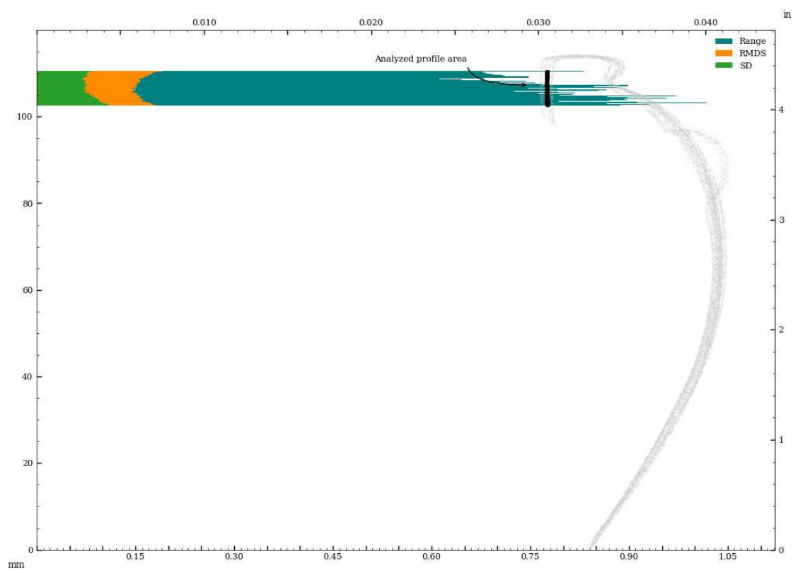
Figure 66: Circularity of interior_separate surface - perpendicular to surface curvature.
