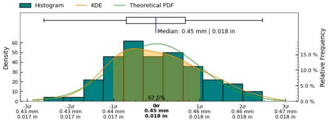
Figure 20: Standard Deviation measurement distribution across measured slices of “ + interior + ” surface
