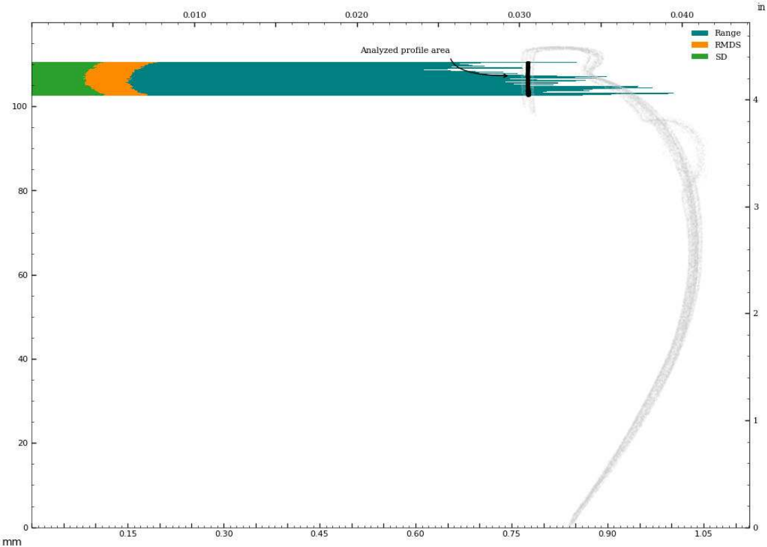
Figure 67: Circularity of interior_separate surface - in z-plane.
