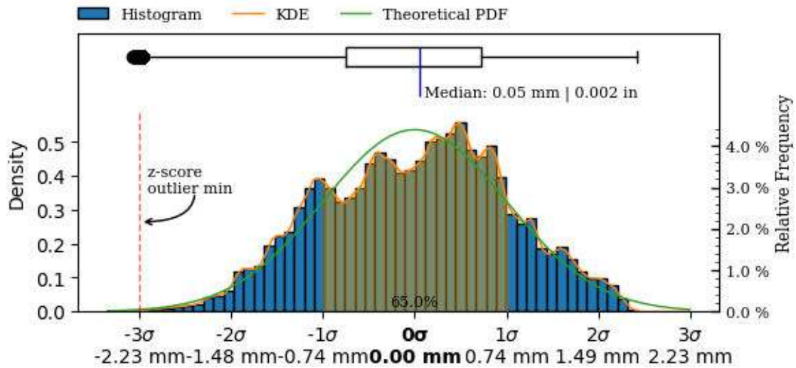
Figure 51: Exterior surface variability boxplot, kds and histogram.
