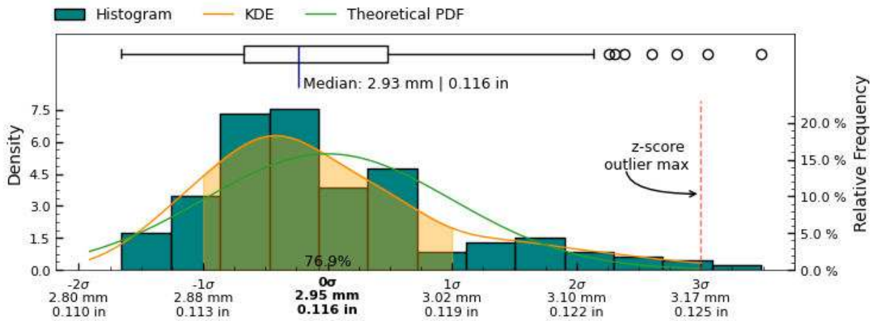
Figure 19: Range measurement distribution across measured slices of interior surface
