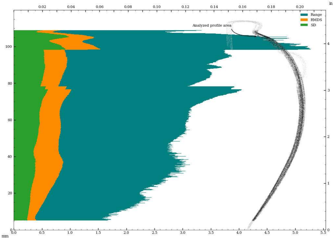
Figure 59: Circularity of exterior surface - in z-plane.
