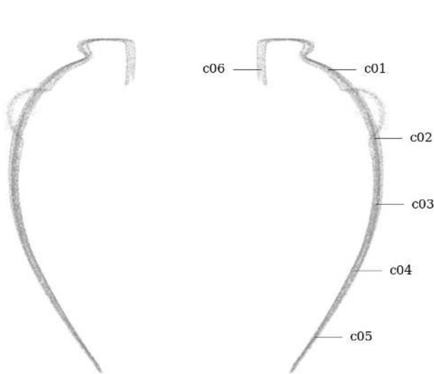
Figure 54: Circularity measurement sample locations, full mesh aligned to exterior surface
