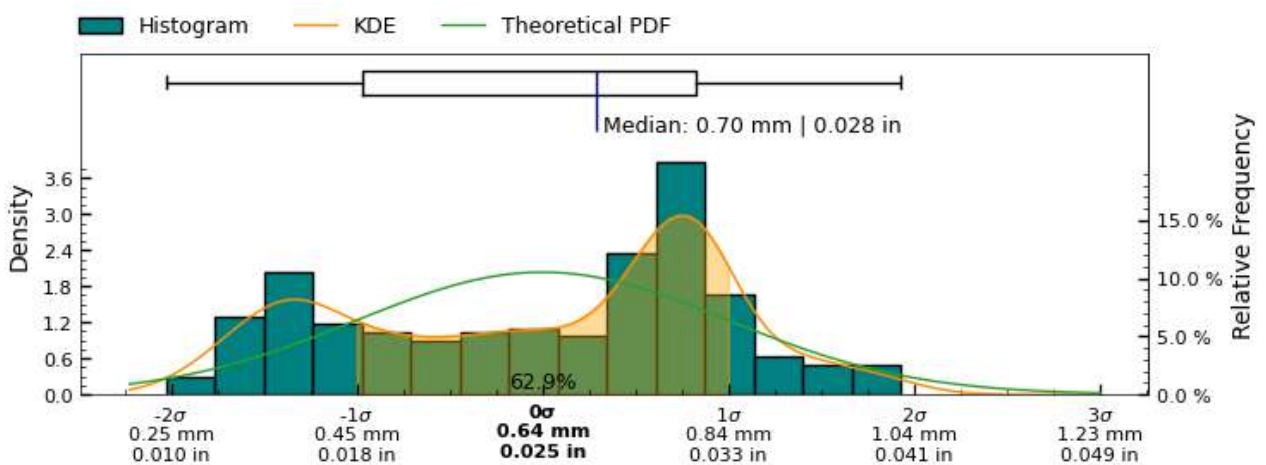
Figure 16: Root Mean Squared Deviation measurement distribution across measured slices of exterior surface
