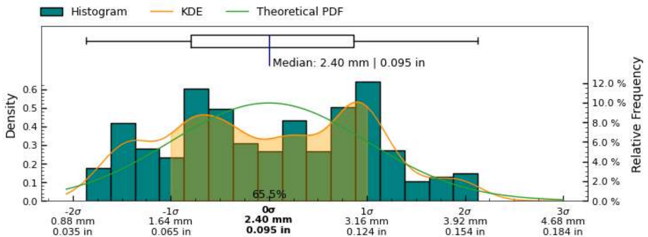
Figure 14: Range measurement distribution across measured slices of exterior surface
