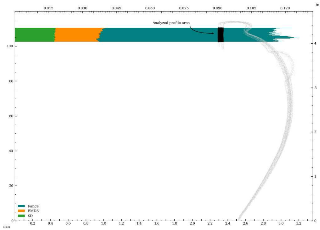
Figure 62: Circularity of interior surface - perpendicular to surface curvature.
