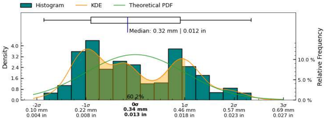
Figure 15: Standard Deviation measurement distribution across measured slices of " + exterior + " surface
