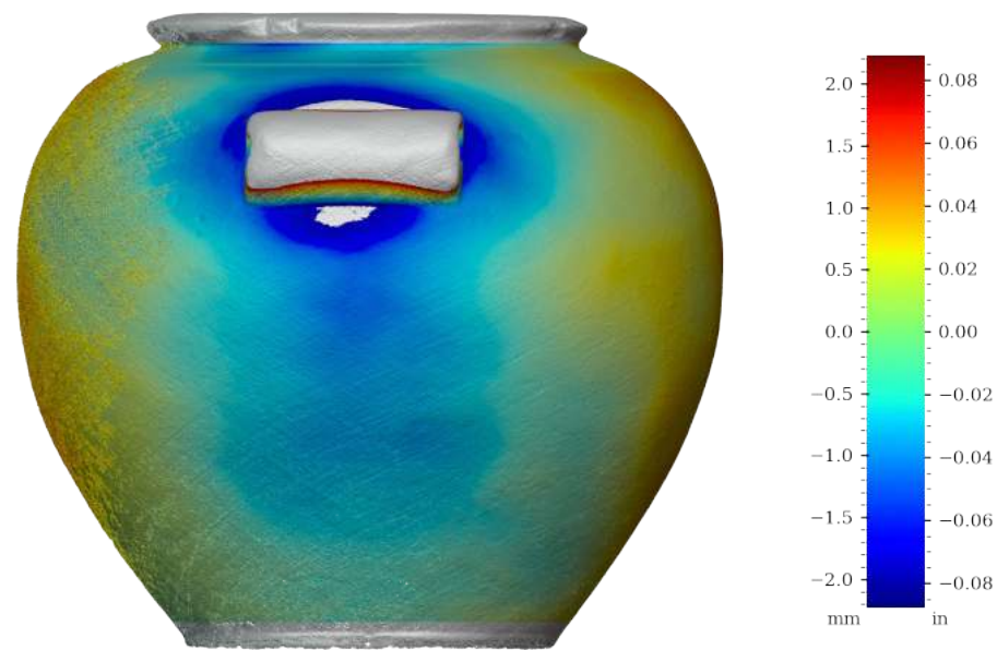
Figure 40: Surface variability heatmap of MV011, rotated 90°
