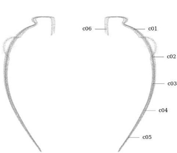
Figure 28: Circularity measurement sample locations, full mesh aligned to exterior surface
