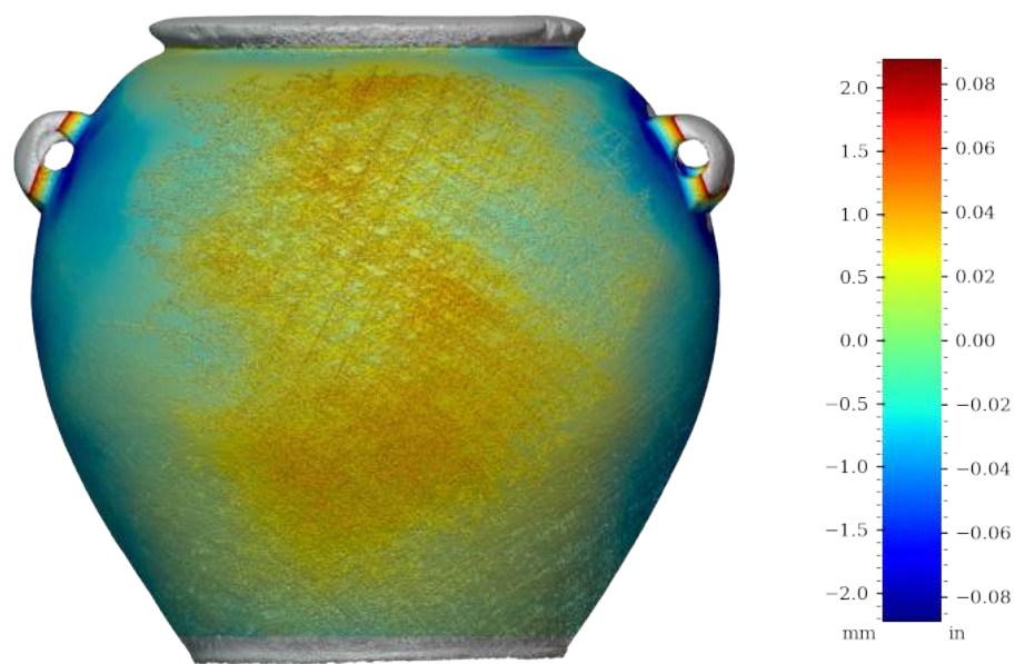
Figure 39: Surface variability heatmap of MV011, front view
