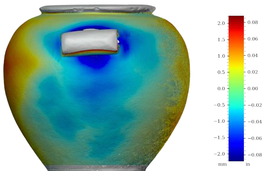
Figure 42: Surface variability heatmap of MV011, rotated 270°
