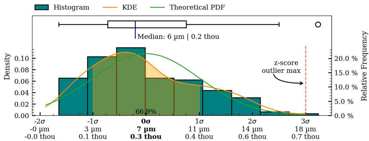
Figure 38: Coaxiality residual plots of interior_separate surface, MV011.
