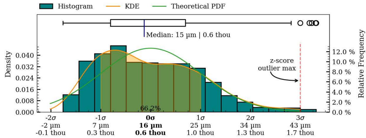
Figure 39: Coaxiality residual plots of interior surface, MV012.
