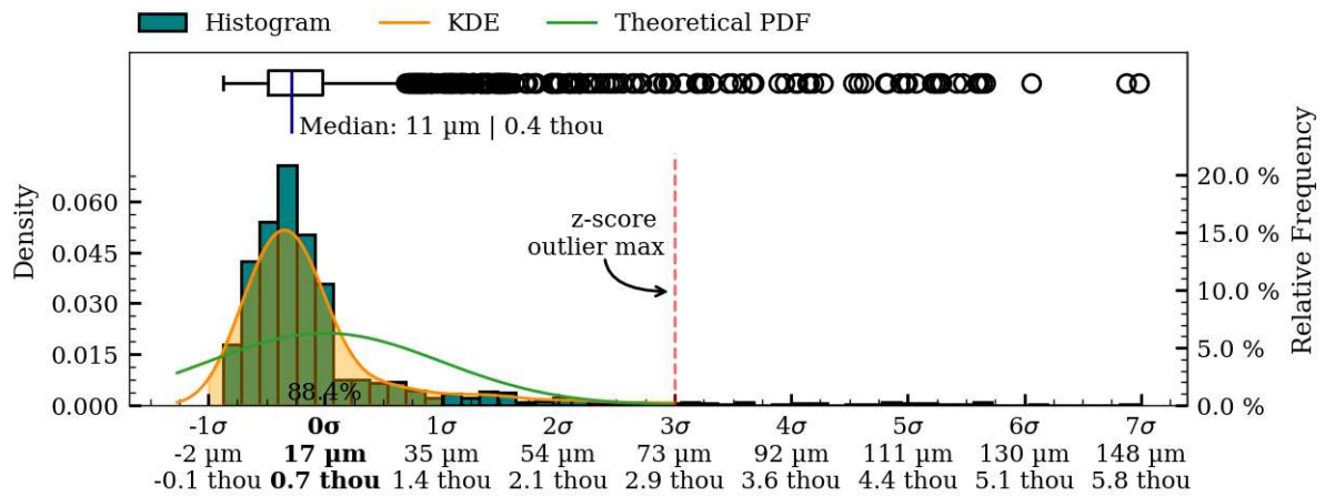
Figure 56: Coaxiality residual plots of interior_separate surface, MV013.
