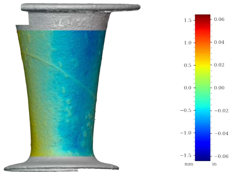
Figure 60: Surface variability heatmap of MV013, rotated 270°
