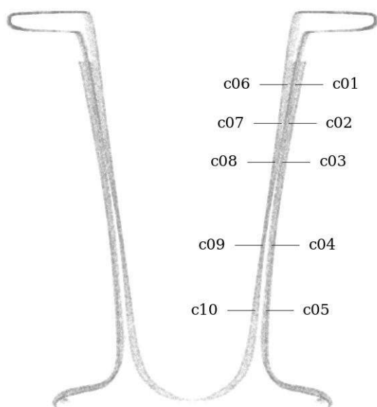
Figure 90: Circularity measurement sample locations, full mesh aligned to exterior surface
