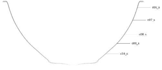
Figure 89: Circularity measurement sample location, separately aligned interior mesh
