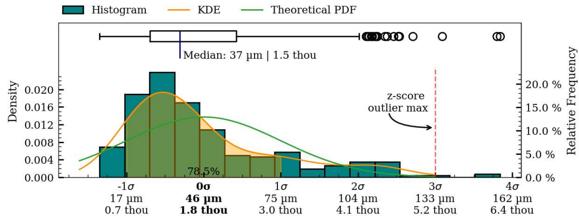
Figure 46: Coaxiality residual plots of exterior surface, MV015c.
