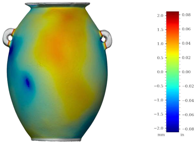
Figure 43: Surface variability heatmap of MV016, rotated 180°
