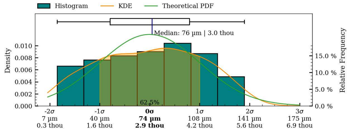
Figure 39: Coaxiality residual plots of interior surface, MV016.
