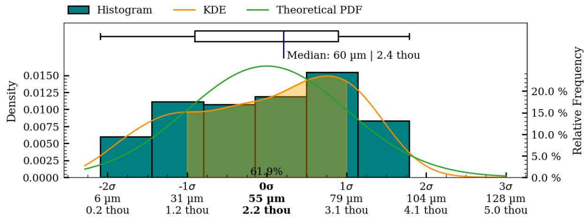
Figure 40: Coaxiality residual plots of interior_separate surface, MV016.
