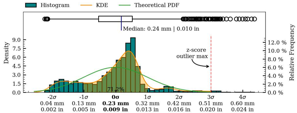
Figure 38: Coaxiality residual plots of exterior surface, MV016.
