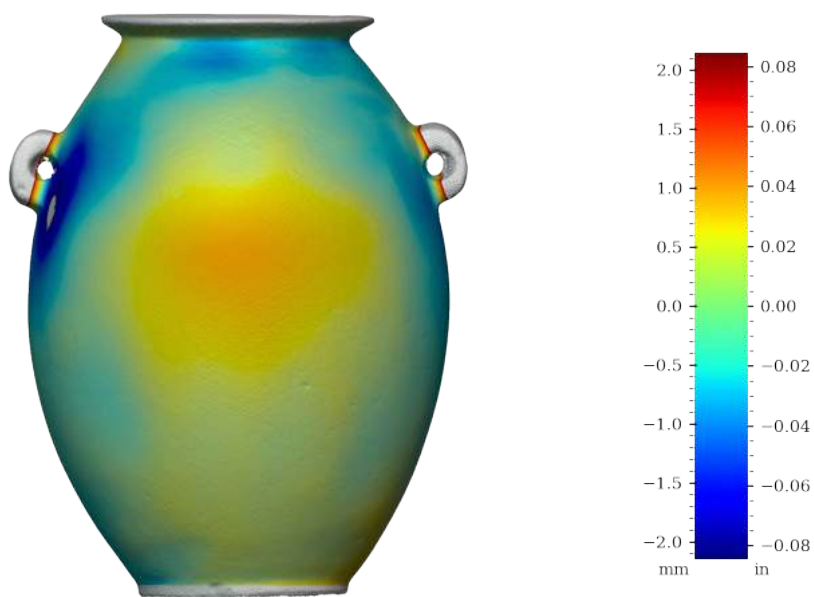
Figure 41: Surface variability heatmap of MV016, front view
