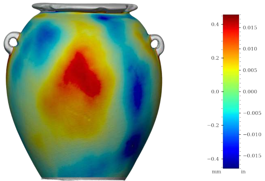
Figure 43: Surface variability heatmap of MV017, rotated 180°
