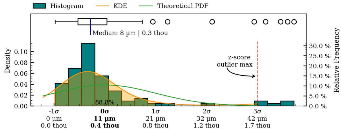
Figure 39: Coaxiality residual plots of interior surface, MV017.
