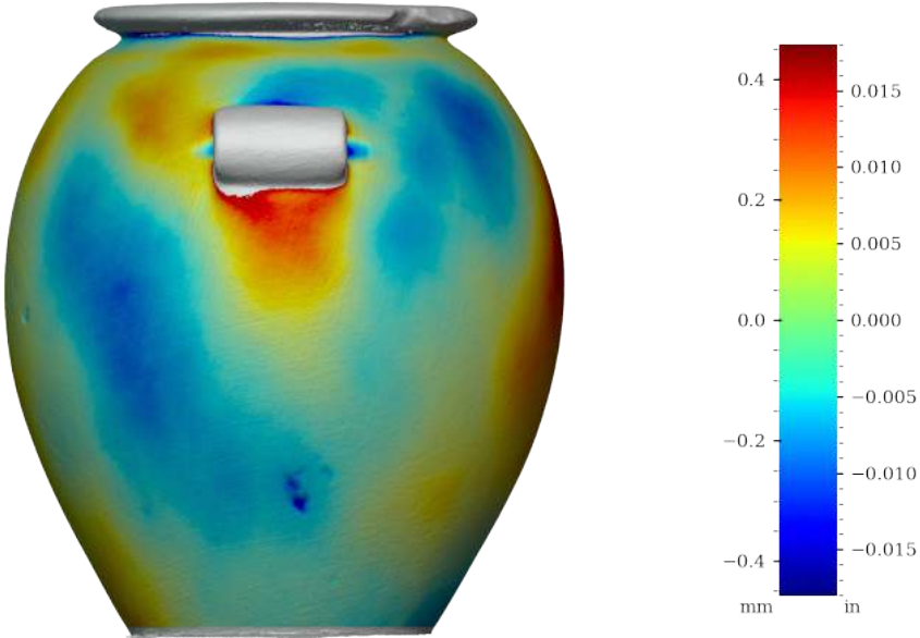
Figure 42: Surface variability heatmap of MV017, rotated 90°
