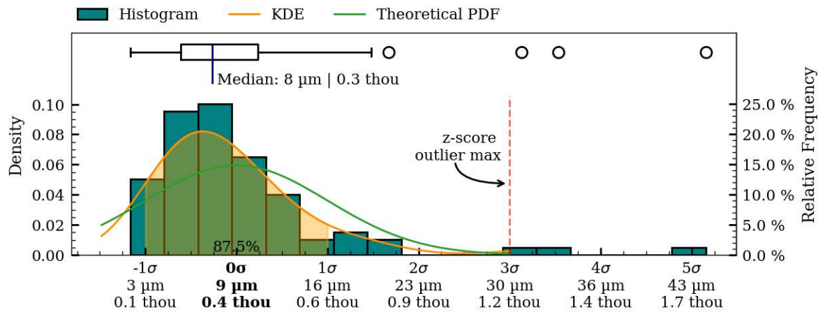
Figure 40: Coaxiality residual plots of interior_separate surface, MV017.
