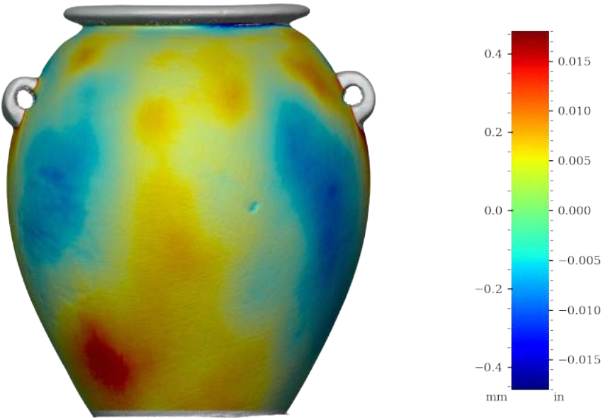
Figure 41: Surface variability heatmap of MV017, front view
