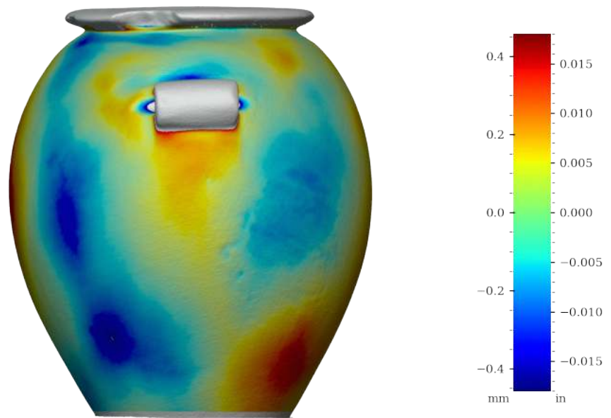
Figure 44: Surface variability heatmap of MV017, rotated 270°
