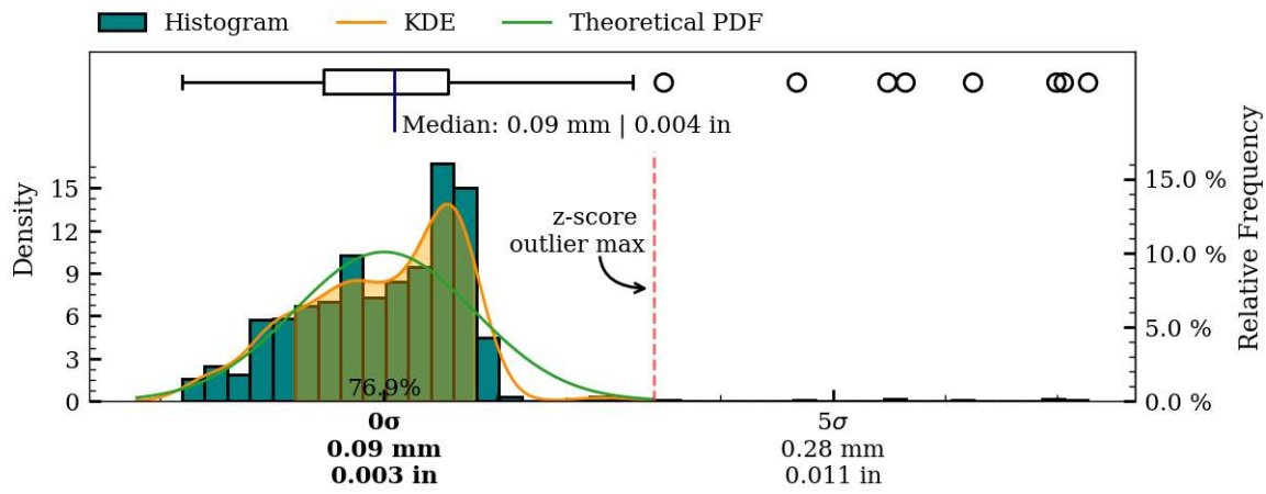
Figure 38: Coaxiality residual plots of exterior surface, MV017.
