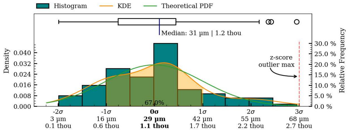
Figure 40: Coaxiality residual plots of interior_separate surface, MV018.
