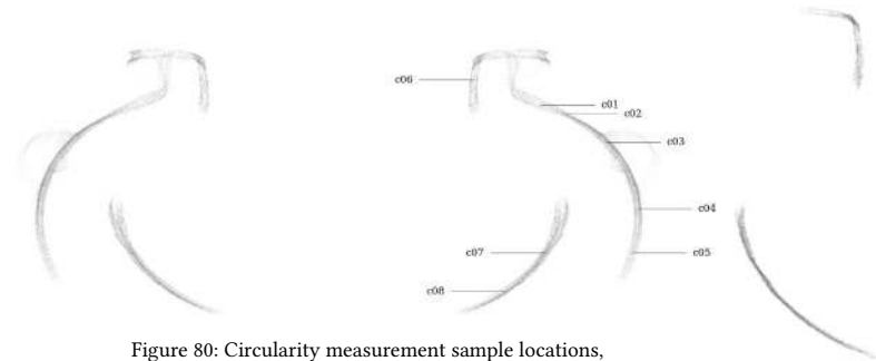
Figure 80: Circularity measurement sample locations, full mesh aligned to exterior surface
