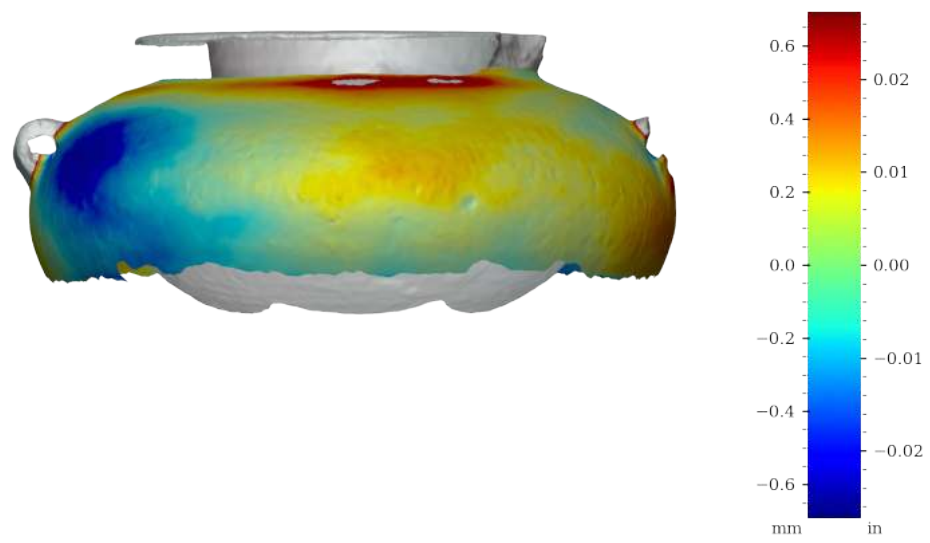
Figure 51: Surface variability heatmap of MV018b, rotated 180°
