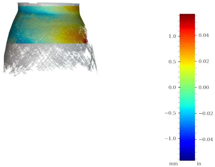
Figure 48: Surface variability heatmap of MV019, rotated 270°
