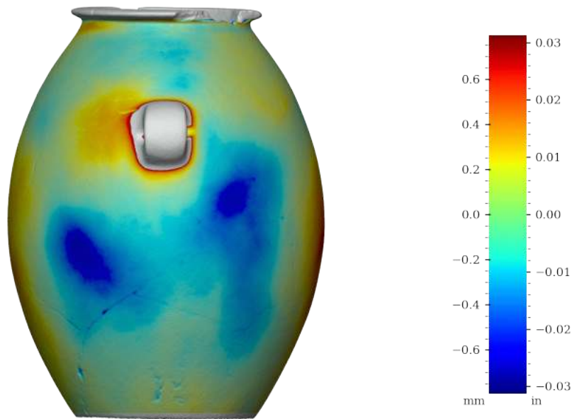
Figure 44: Surface variability heatmap of MV019, rotated 270°
