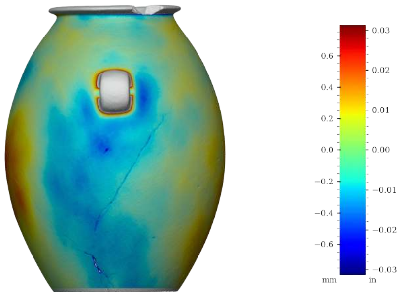
Figure 42: Surface variability heatmap of MV019, rotated 90°
