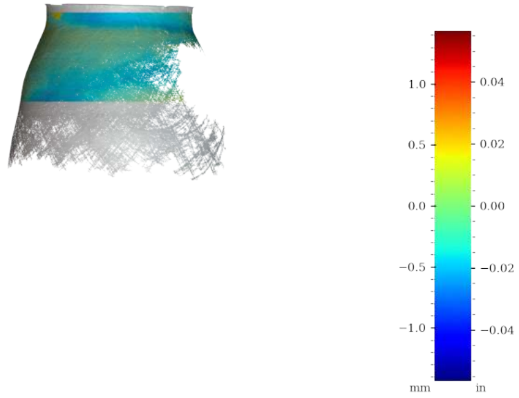
Figure 47: Surface variability heatmap of MV019, rotated 180°
