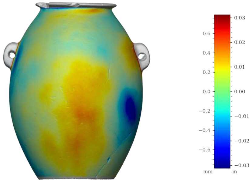
Figure 43: Surface variability heatmap of MV019, rotated 180°
