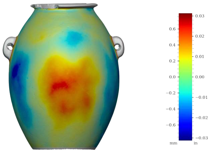
Figure 41: Surface variability heatmap of MV019, front view
