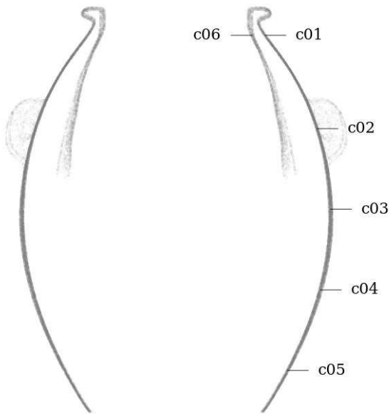
Figure 72: Circularity measurement sample locations, full mesh aligned to exterior surface
