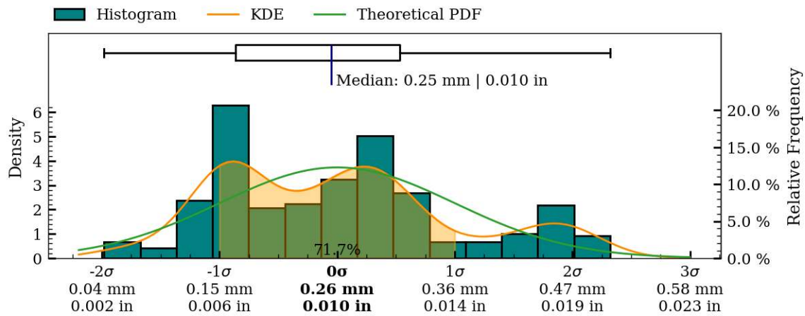
Figure 39: Coaxiality residual plots of interior surface, MV019.
