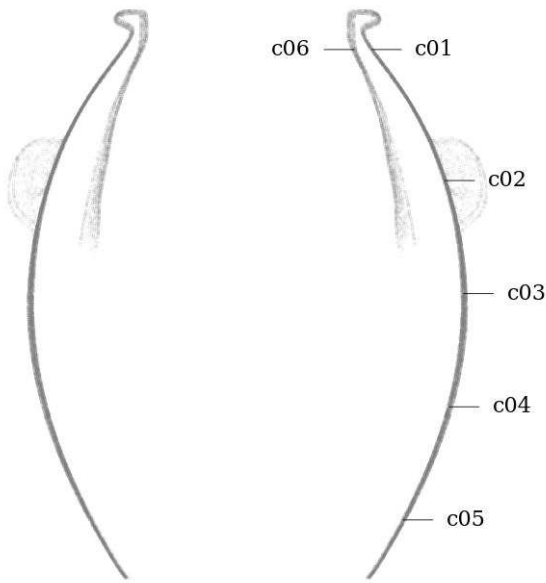
Figure 74: Circularity measurement sample locations, full mesh aligned to exterior surface
