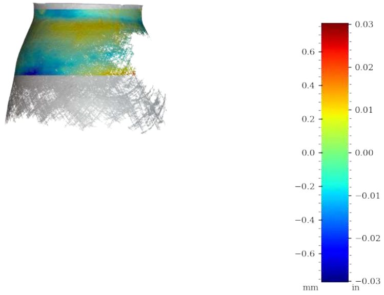
Figure 51: Surface variability heatmap of MV019, rotated 180°
