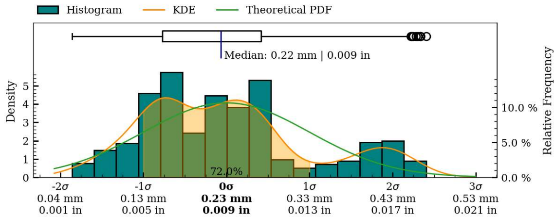
Figure 40: Coaxiality residual plots of interior_separate surface, MV019.
