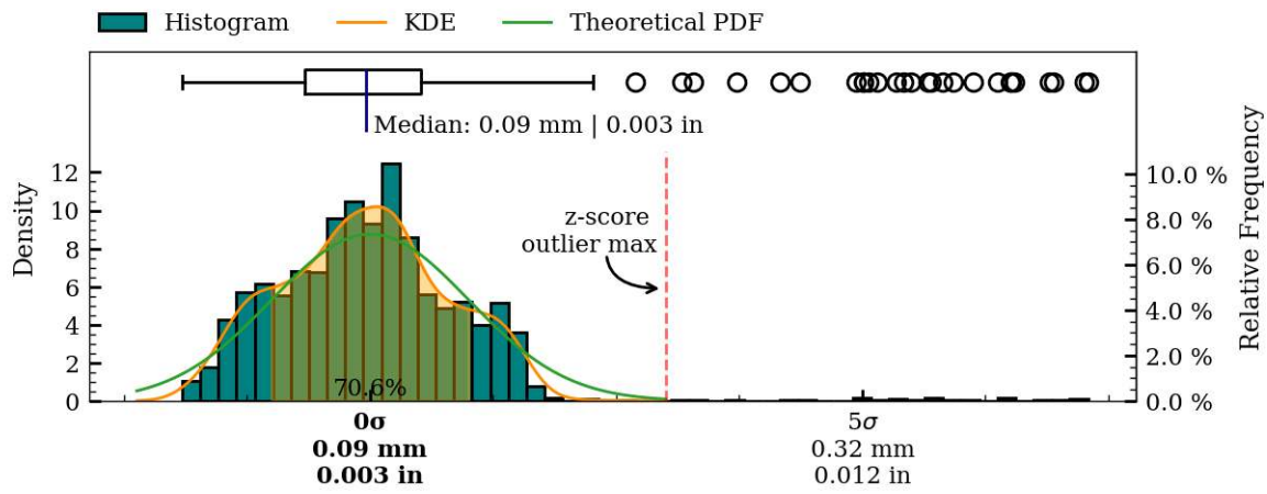
Figure 38: Coaxiality residual plots of exterior surface, MV019.
