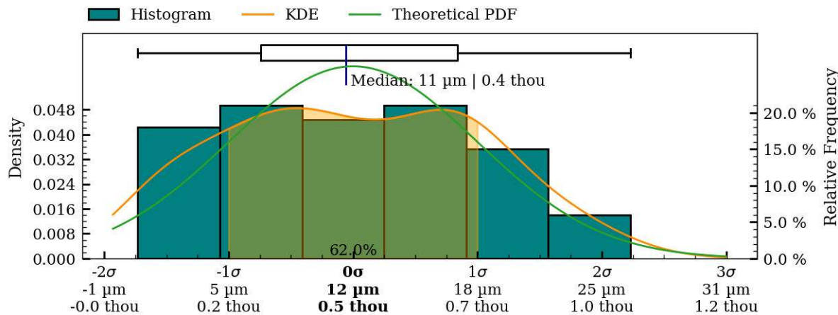
Figure 40: Coaxiality residual plots of interior_separate surface, MV020.
