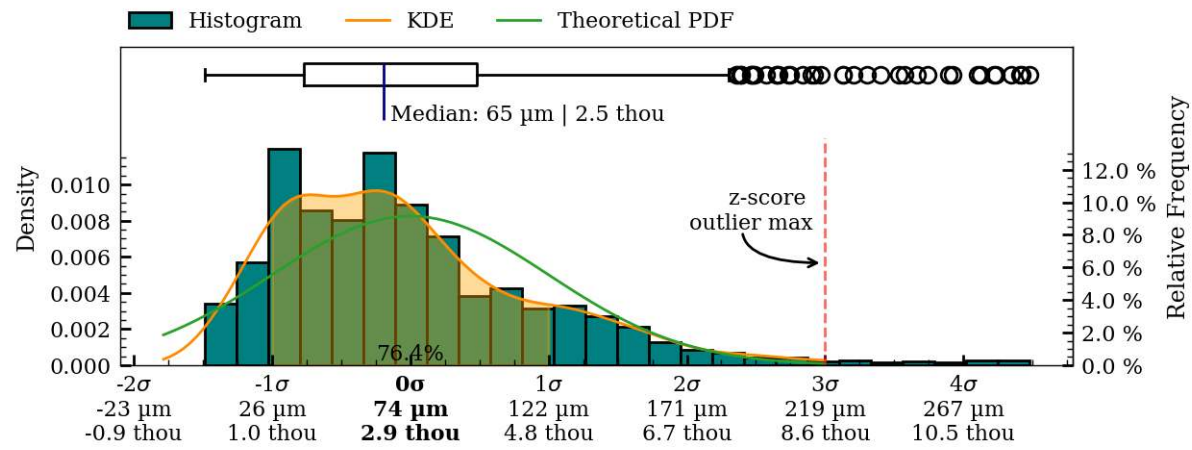
Figure 38: Coaxiality residual plots of exterior surface, MV020.
