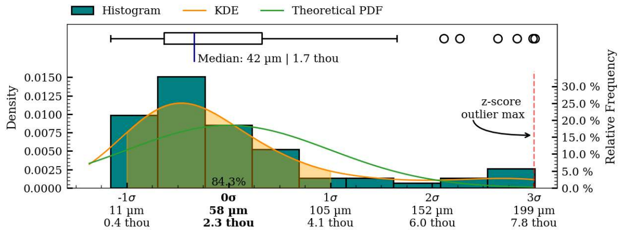
Figure 40: Coaxiality residual plots of interior_separate surface, MV020b.
