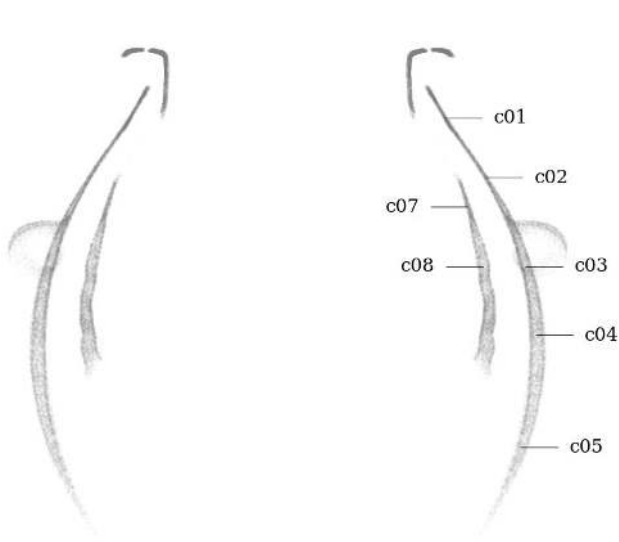
Figure 29: Circularity measurement sample locations, full mesh aligned to exterior surface
