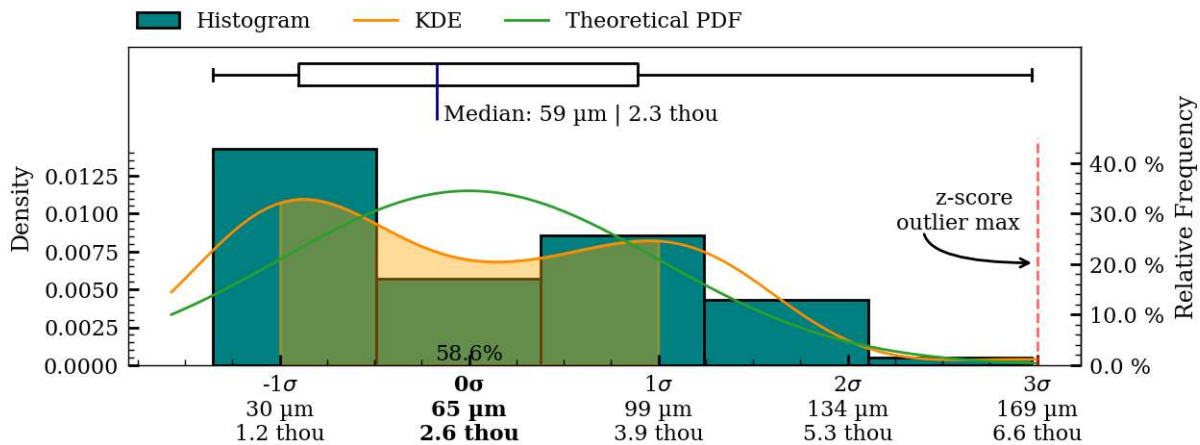
Figure 39: Coaxiality residual plots of interior surface, MV020b.
