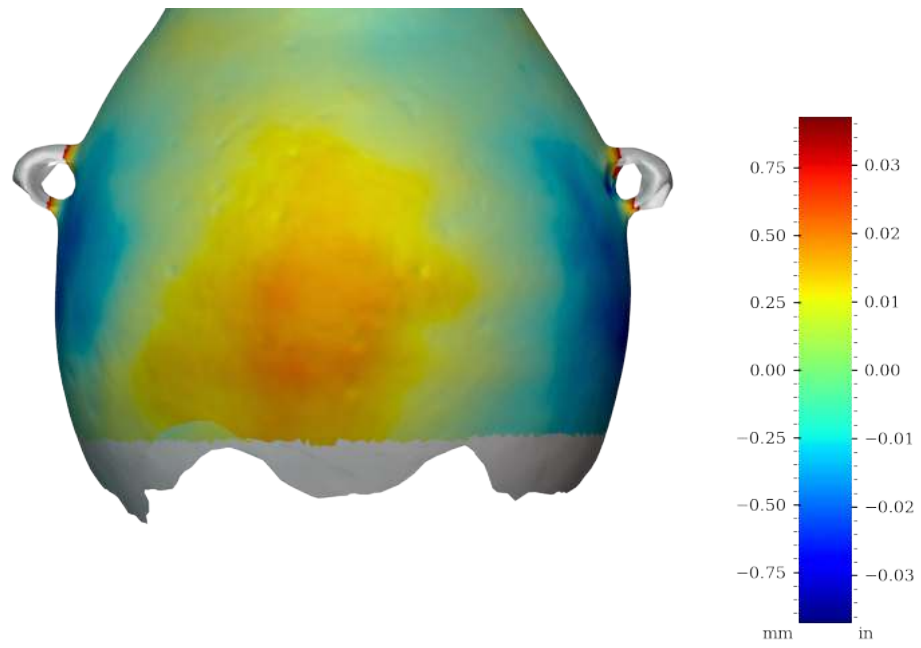
Figure 43: Surface variability heatmap of MV020b, rotated 180°
