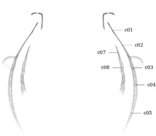
Figure 58: Circularity measurement sample locations, full mesh aligned to exterior surface
