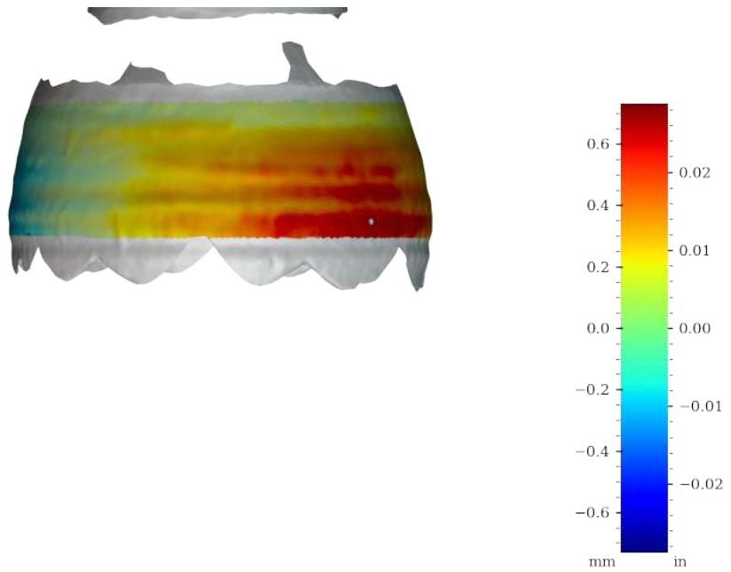
Figure 48: Surface variability heatmap of MV020b, rotated 270°
