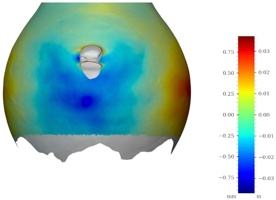
Figure 44: Surface variability heatmap of MV020b, rotated 270°
