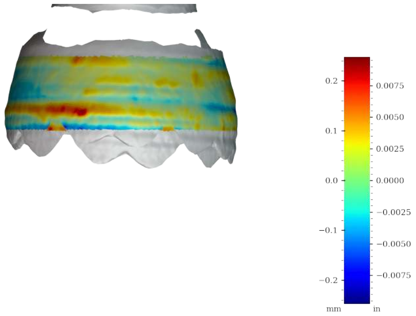
Figure 51: Surface variability heatmap of MV020b, rotated 180°
