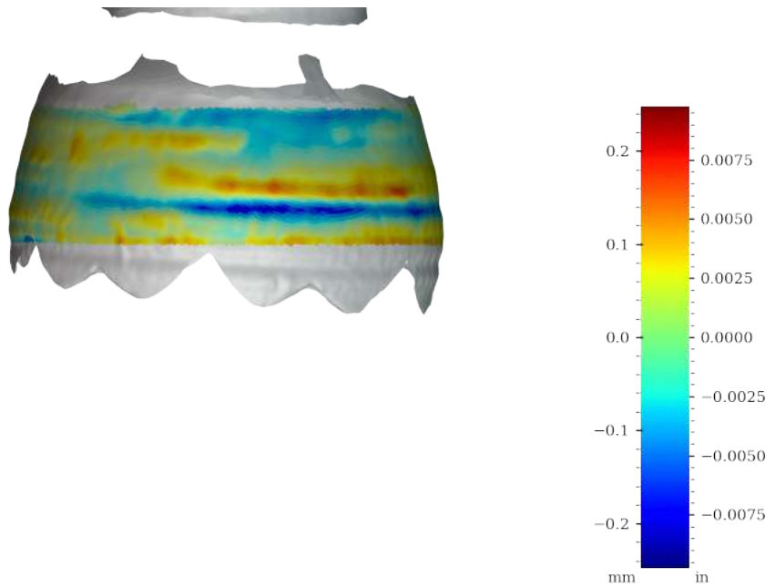
Figure 52: Surface variability heatmap of MV020b, rotated 270°
