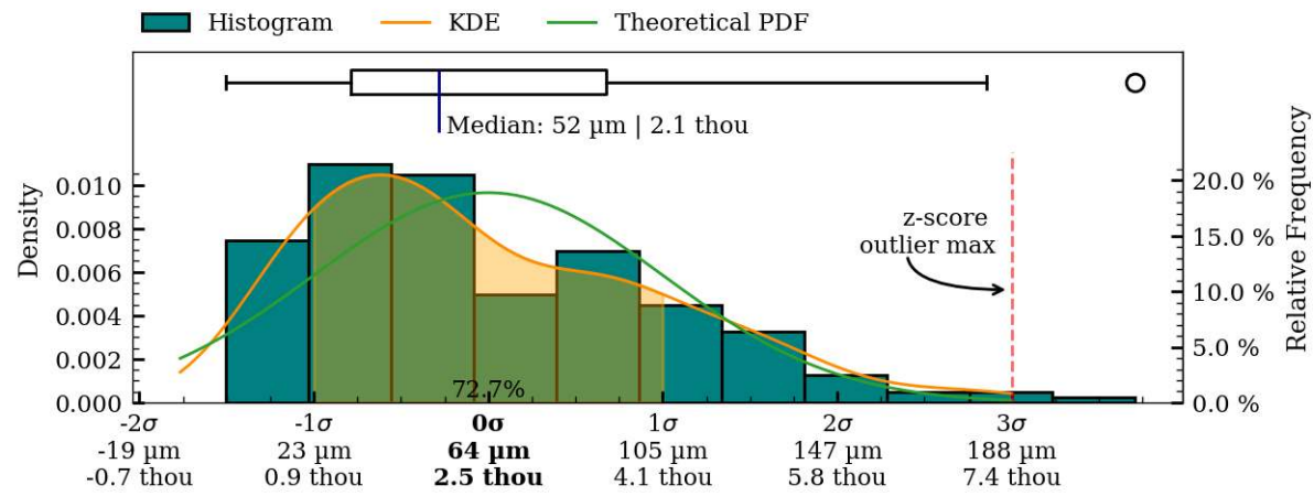
Figure 38: Coaxiality residual plots of exterior surface, MV020b.
