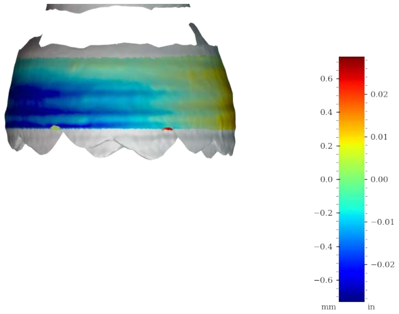
Figure 47: Surface variability heatmap of MV020b, rotated 180°
