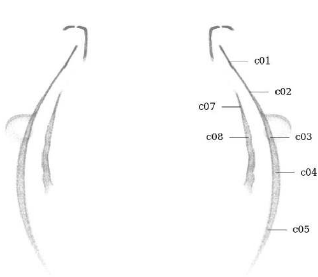
Figure 74: Circularity measurement sample locations, full mesh aligned to exterior surface
