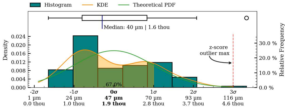
Figure 40: Coaxiality residual plots of interior_separate surface, MV021.
