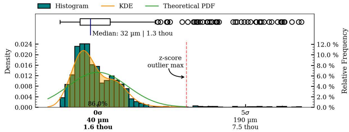
Figure 38: Coaxiality residual plots of exterior surface, MV021.
