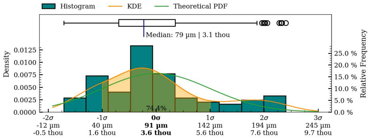
Figure 51: Coaxiality residual plots of interior surface, MV021b.
