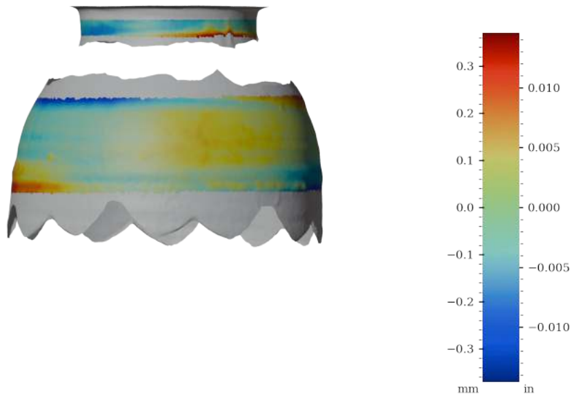
Figure 63: Surface variability heatmap of MV021b, rotated 180°
