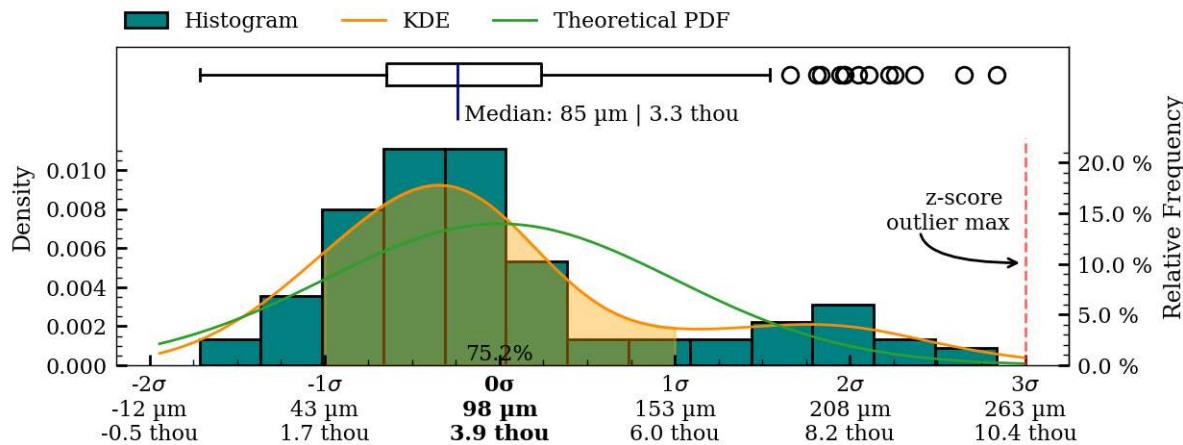
Figure 52: Coaxiality residual plots of interior_separate surface, MV021b.
