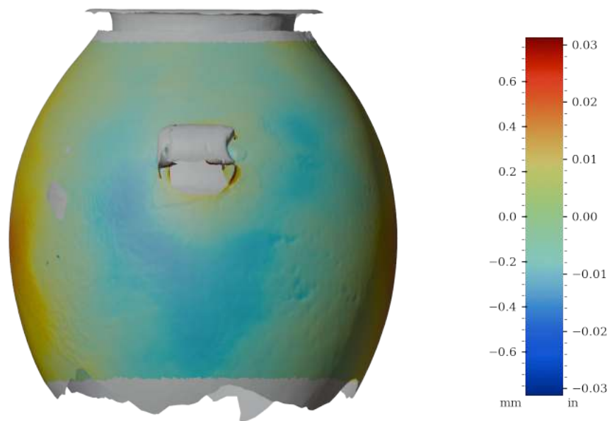
Figure 56: Surface variability heatmap of MV021b, rotated 270°
