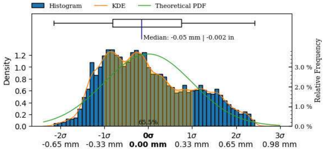
Figure 65: Exterior surface variability boxplot, kds and histogram.
