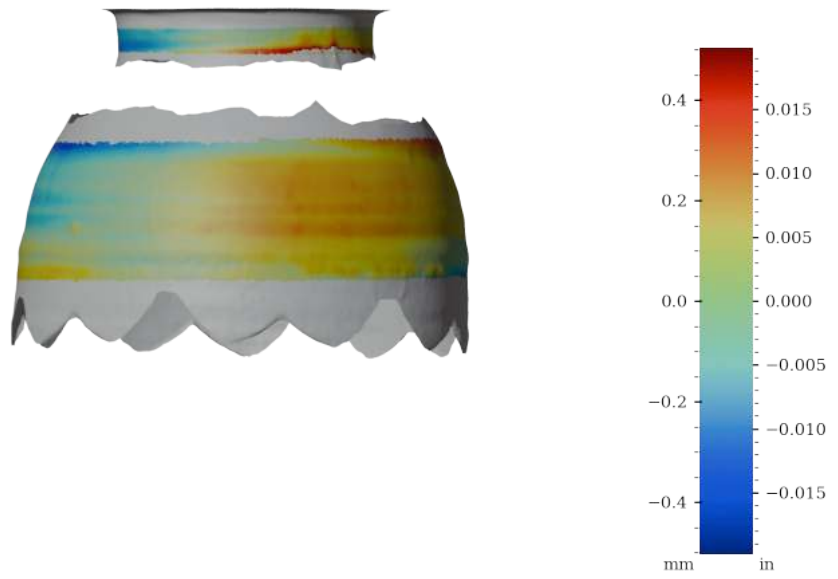
Figure 59: Surface variability heatmap of MV021b, rotated 180°
