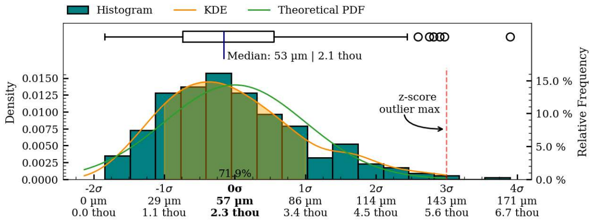
Figure 50: Coaxiality residual plots of exterior surface, MV021b.
