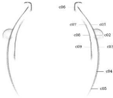
Figure 68: Circularity measurement sample locations, full mesh aligned to exterior surface
