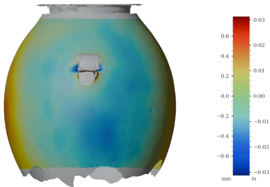
Figure 54: Surface variability heatmap of MV021b, rotated 90°
