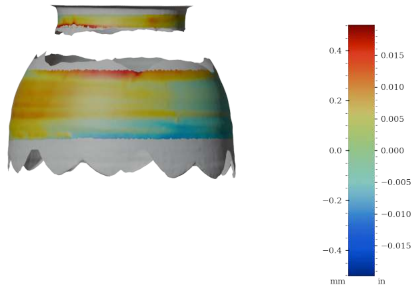
Figure 60: Surface variability heatmap of MV021b, rotated 270°
