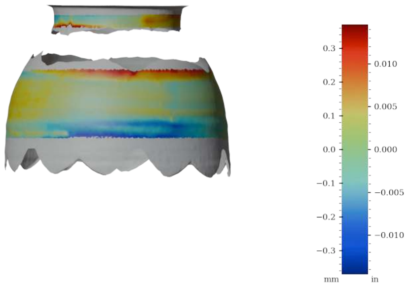
Figure 64: Surface variability heatmap of MV021b, rotated 270°
