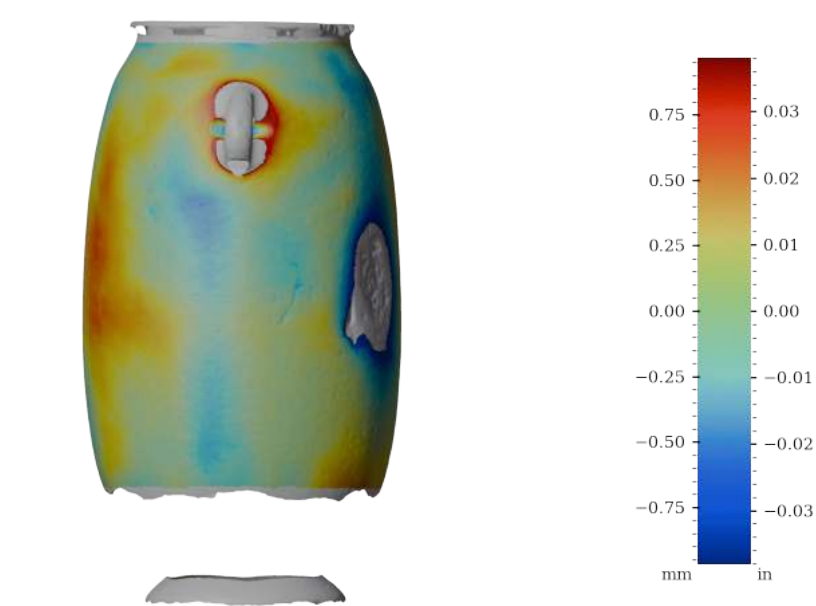
Figure 50: Surface variability heatmap of MV022, rotated 90°
