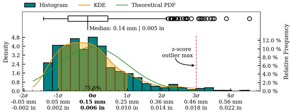
Figure 46: Coaxiality residual plots of exterior surface, MV022.
