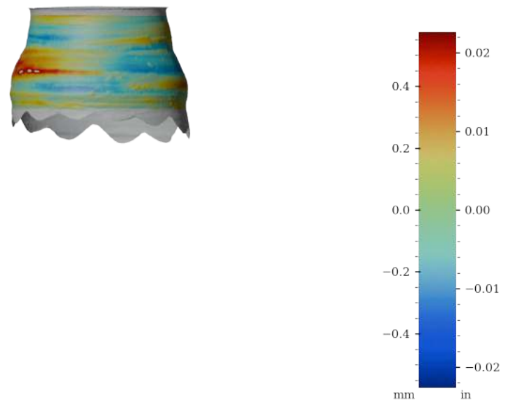
Figure 60: Surface variability heatmap of MV022, rotated 270°
