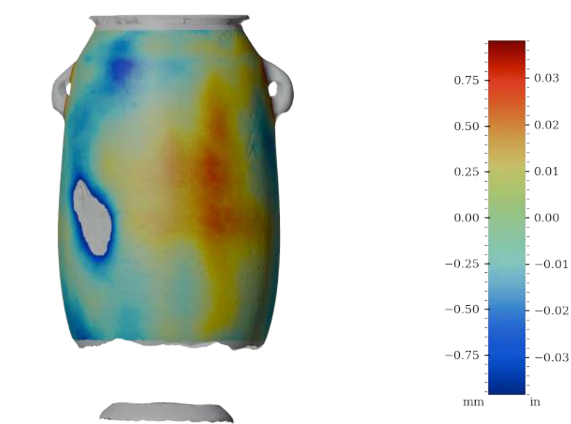
Figure 49: Surface variability heatmap of MV022, front view
