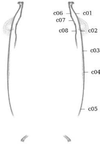
Figure 64: Circularity measurement sample locations, full mesh aligned to exterior surface
