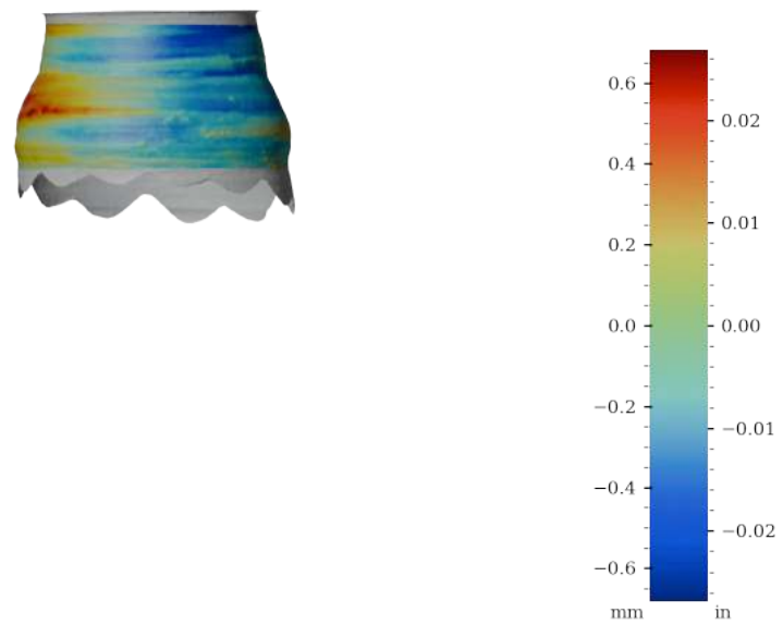
Figure 56: Surface variability heatmap of MV022, rotated 270°
