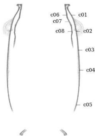
Figure 82: Circularity measurement sample locations, full mesh aligned to exterior surface
