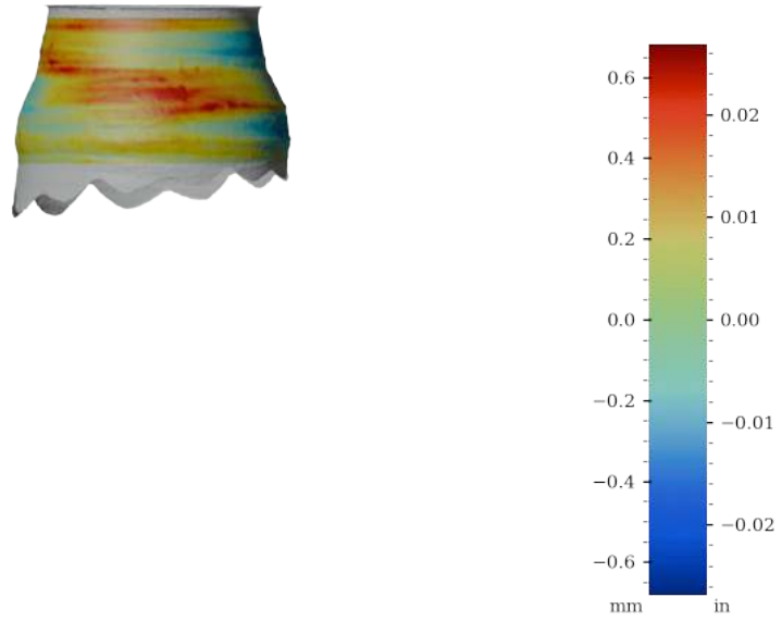
Figure 55: Surface variability heatmap of MV022, rotated 180°
