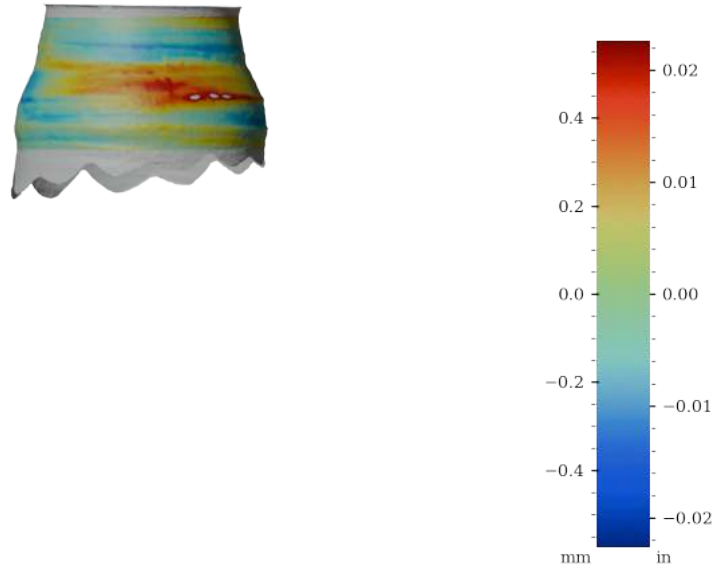
Figure 59: Surface variability heatmap of MV022, rotated 180°
