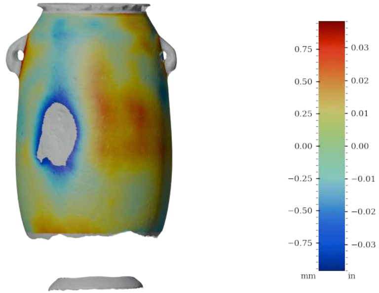
Figure 51: Surface variability heatmap of MV022, rotated 180°
