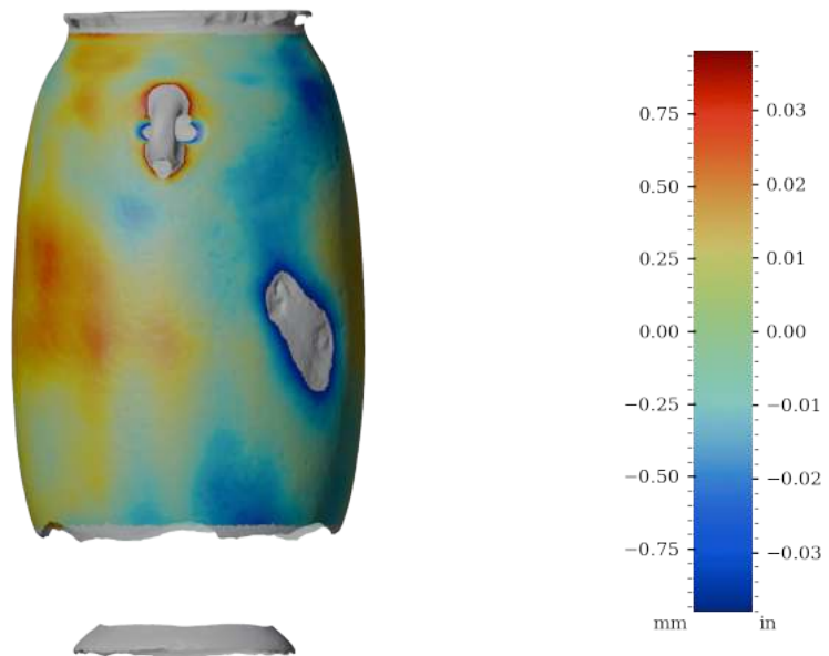
Figure 52: Surface variability heatmap of MV022, rotated 270°
