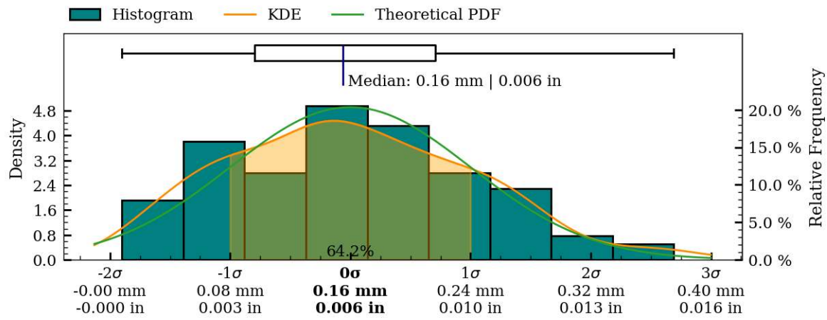
Figure 47: Coaxiality residual plots of interior surface, MV022.
