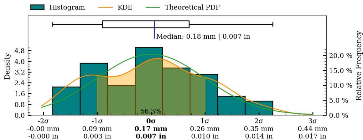
Figure 48: Coaxiality residual plots of interior_separate surface, MV022.
