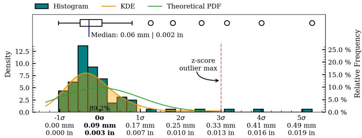
Figure 43: Coaxiality residual plots of interior surface, MV023.
