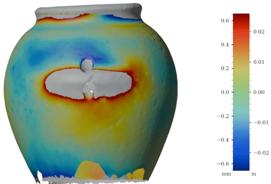
Figure 48: Surface variability heatmap of MV023, rotated 270°
