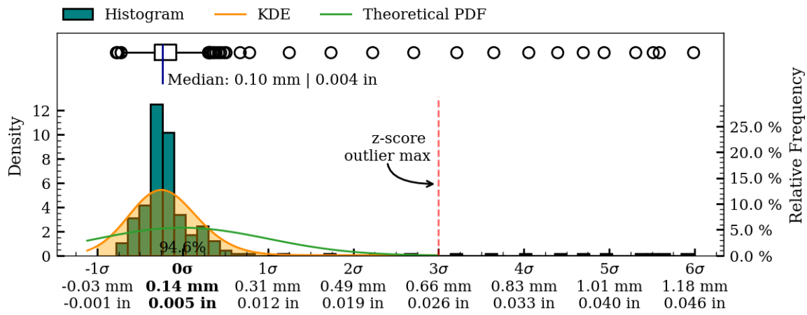
Figure 42: Coaxiality residual plots of exterior surface, MV023.
