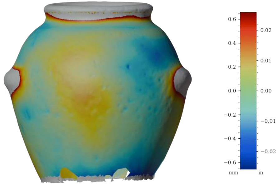
Figure 47: Surface variability heatmap of MV023, rotated 180°
