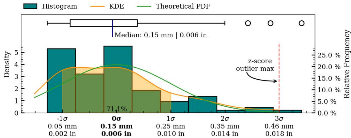
Figure 44: Coaxiality residual plots of interior_separate surface, MV023.
