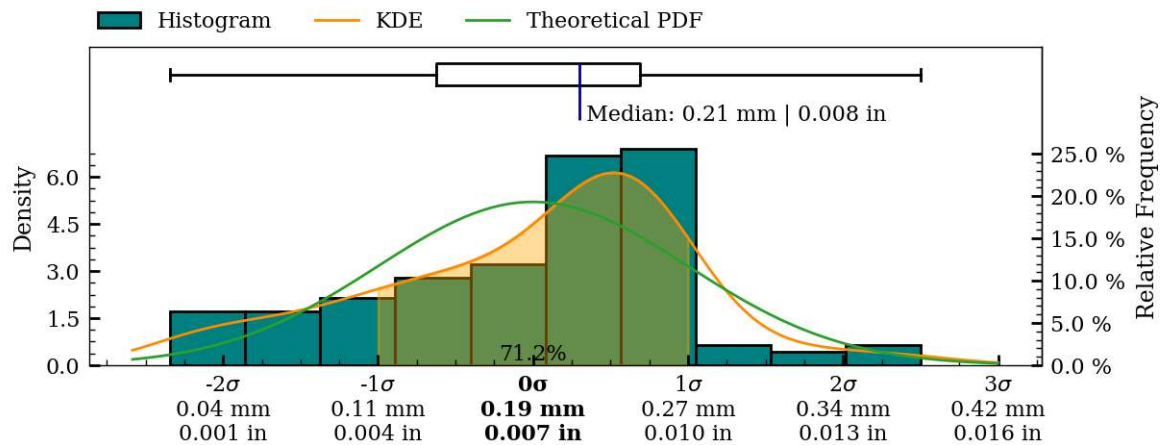
Figure 48: Coaxiality residual plots of interior_separate surface, MV023b.
