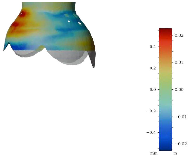
Figure 60: Surface variability heatmap of MV023b, rotated 270°
