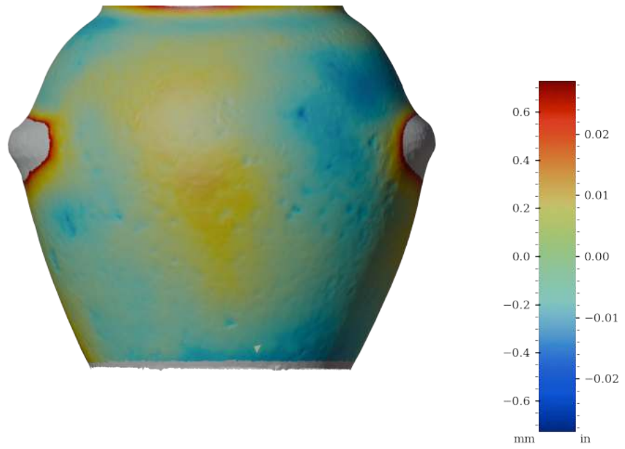
Figure 51: Surface variability heatmap of MV023b, rotated 180°
