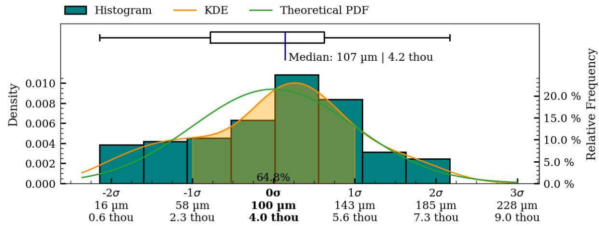
Figure 47: Coaxiality residual plots of interior surface, MV023b.
