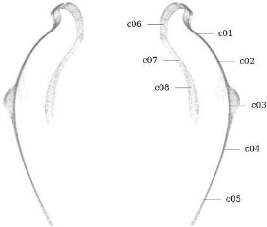
Figure 64: Circularity measurement sample locations, full mesh aligned to exterior surface
