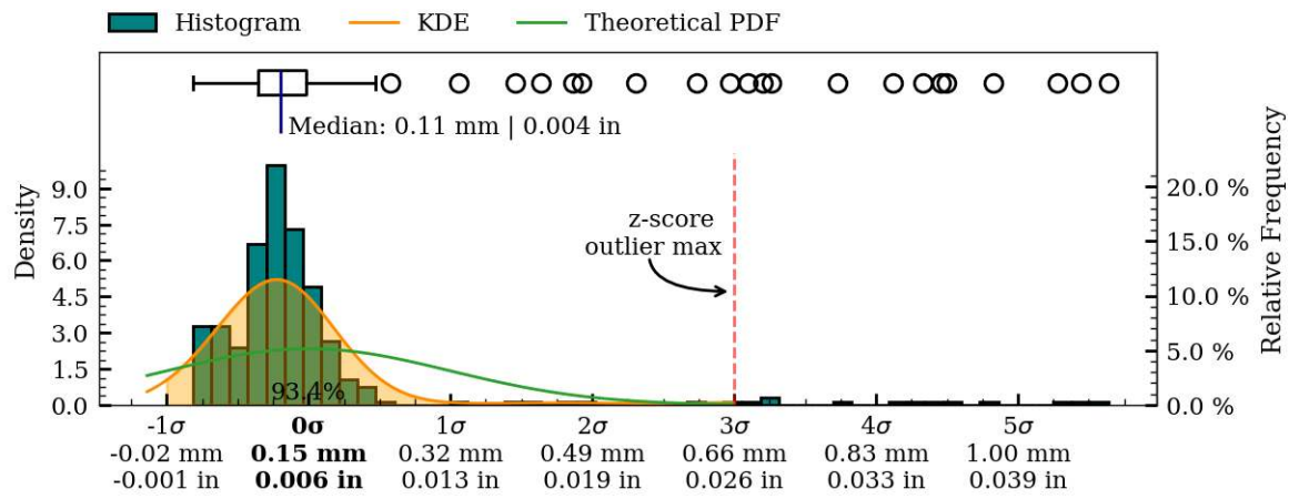
Figure 46: Coaxiality residual plots of exterior surface, MV023b.
