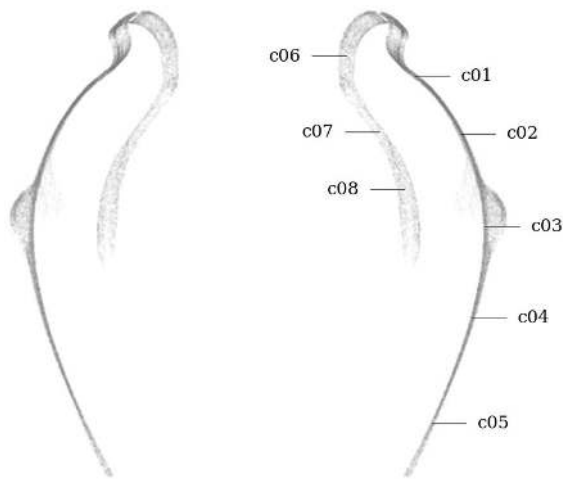
Figure 80: Circularity measurement sample locations, full mesh aligned to exterior surface
