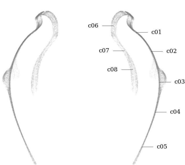
Figure 82: Circularity measurement sample locations, full mesh aligned to exterior surface
