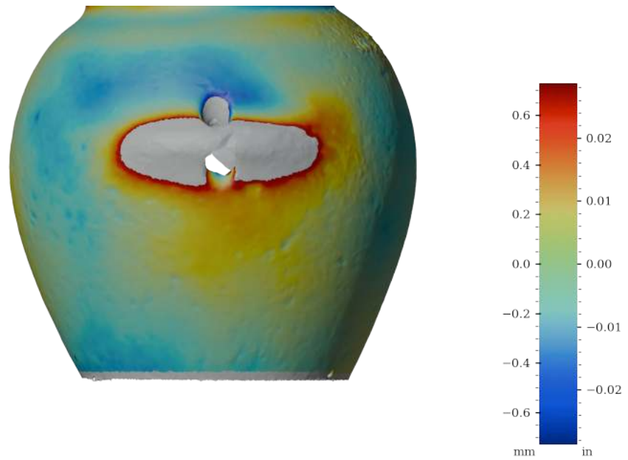
Figure 52: Surface variability heatmap of MV023b, rotated 270°
