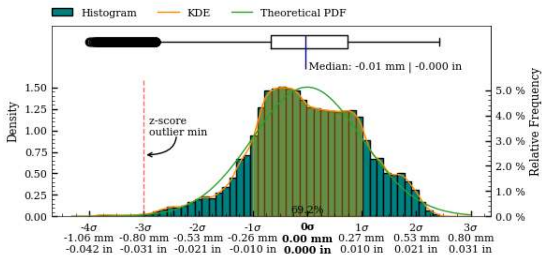
Figure 61: Interior separately aligned surface variability boxplot, kds and histogram.
