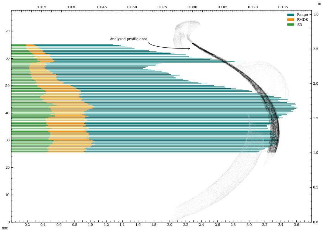
Figure 67: Circularity of exterior surface - in z-plane.
