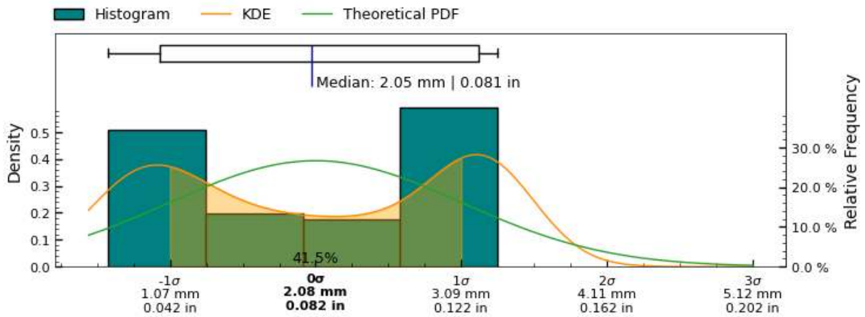
Figure 18: Range measurement distribution across measured slices of exterior surface
