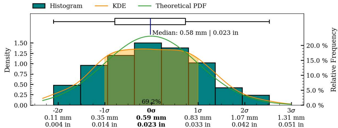
Figure 45: Coaxiality residual plots of interior surface, MV024.
