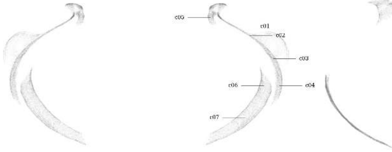
Figure 78: Circularity measurement sample locations, full mesh aligned to exterior surface
