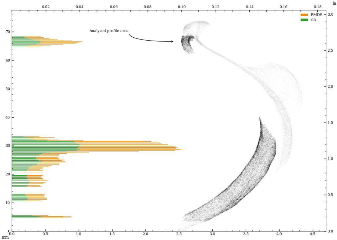
Figure 72: Vessel circularity of interior surface, perpendicular to surface curvature, standard deviation and median absolute deviation.
