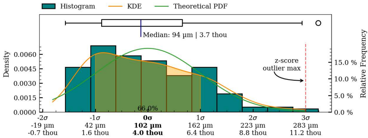
Figure 44: Coaxiality residual plots of exterior surface, MV024.
