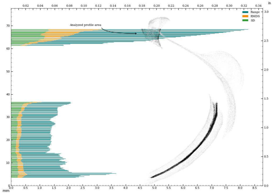
Figure 75: Circularity of interior_separate surface - in z-plane.
