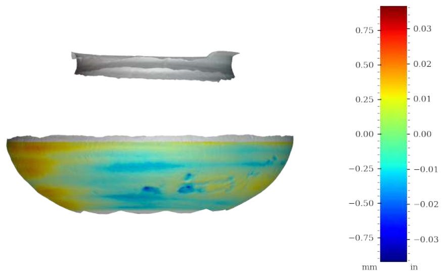
Figure 58: Surface variability heatmap of MV024, rotated 270°
