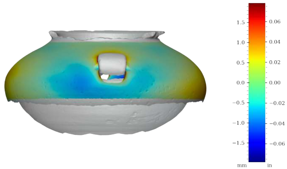
Figure 50: Surface variability heatmap of MV024, rotated 270°
