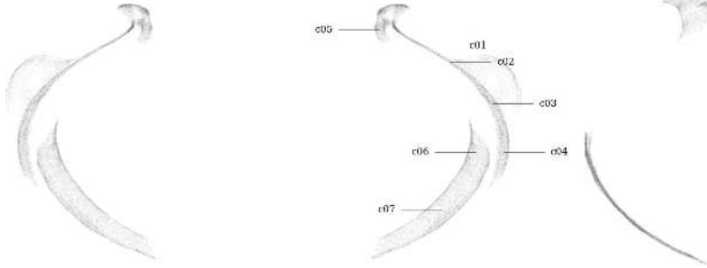
Figure 62: Circularity measurement sample locations, full mesh aligned to exterior surface
