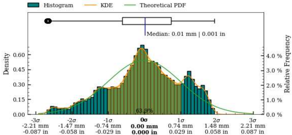
Figure 59: Exterior surface variability boxplot, kds and histogram.
