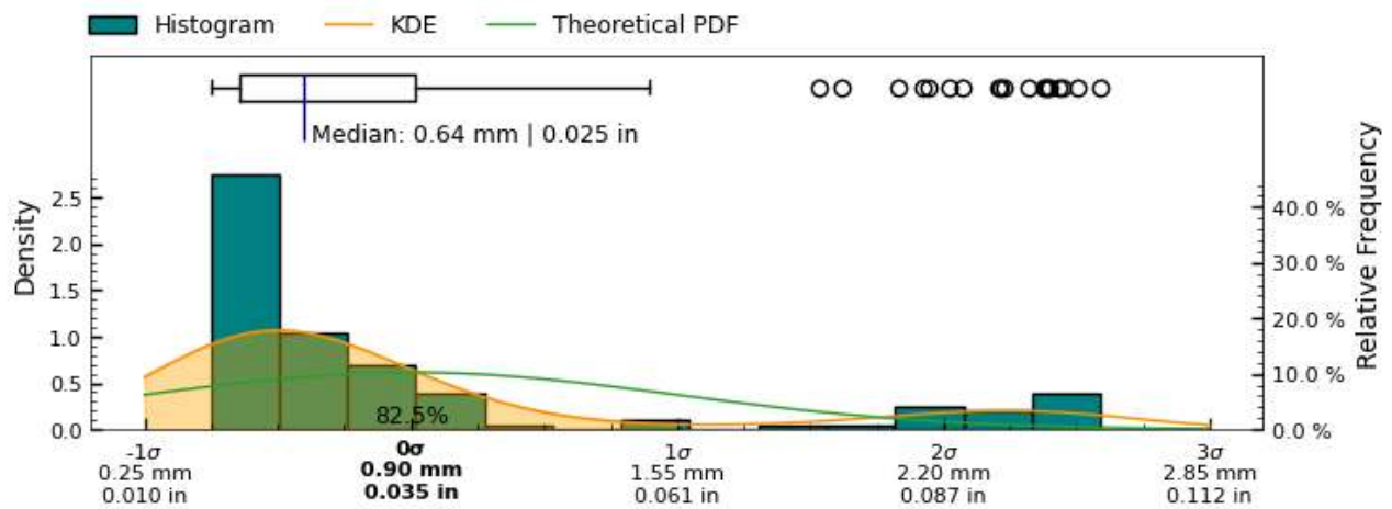
Figure 25: Root Mean Squared Deviation measurement distribution across measured slices of interior surface
