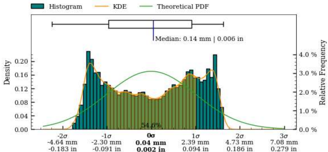
Figure 60: Interior surface variability boxplot, kds and histogram.
