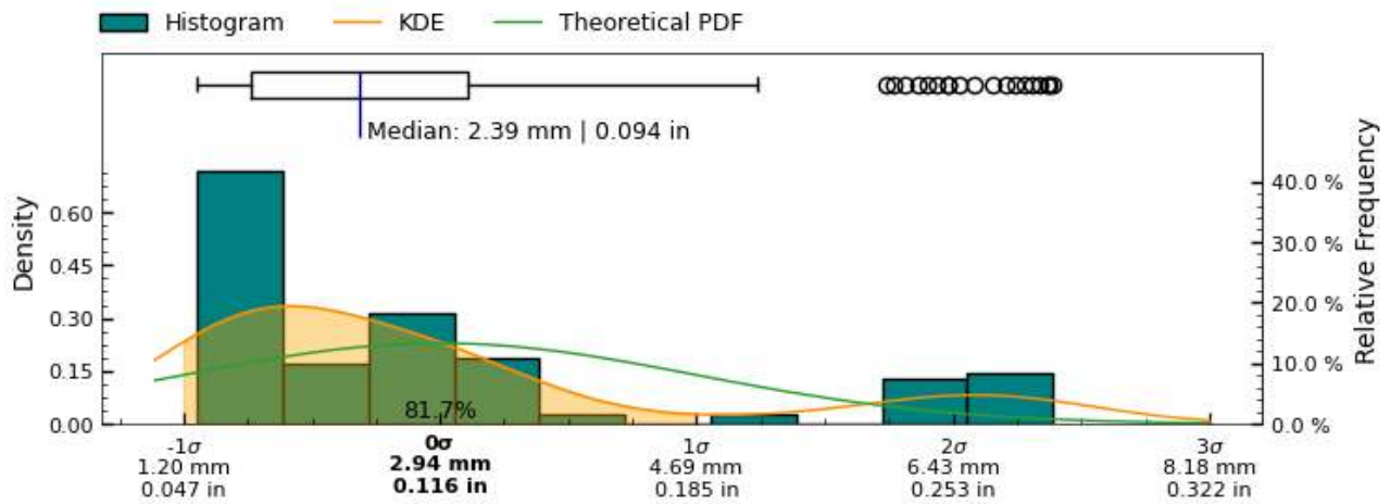
Figure 23: Range measurement distribution across measured slices of interior surface
