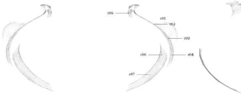
Figure 64: Circularity measurement sample locations, full mesh aligned to exterior surface
