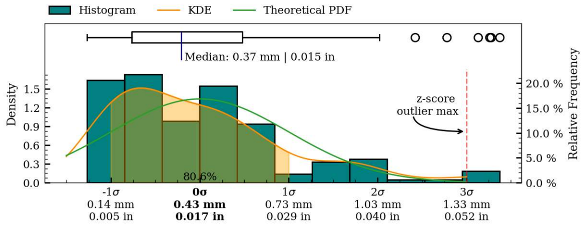
Figure 46: Coaxiality residual plots of interior_separate surface, MV024.
