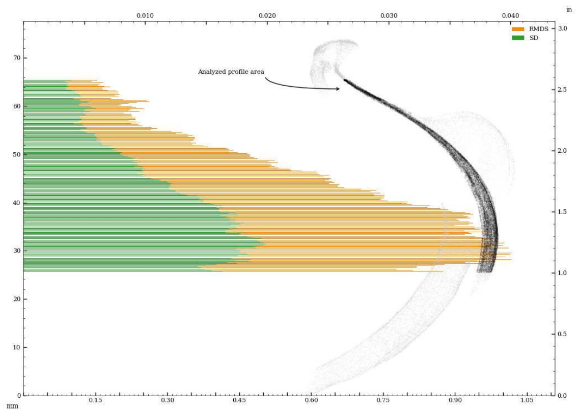
Figure 68: Vessel circularity of exterior surface, perpendicular to surface curvature, standard deviation and median absolute deviation.
