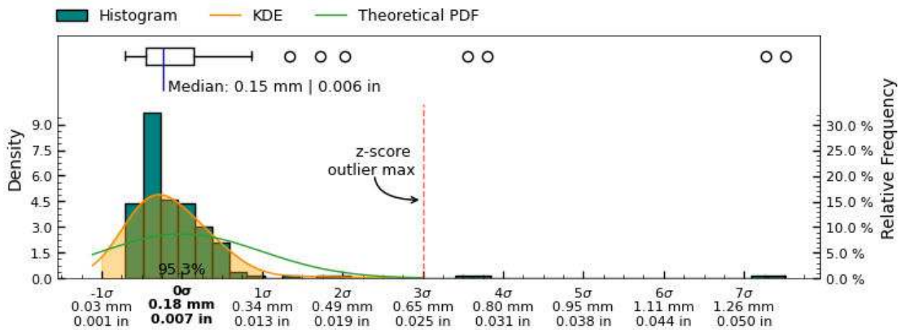
Figure 29: Standard Deviation measurement distribution across measured slices of " + interior_separate + " surface
