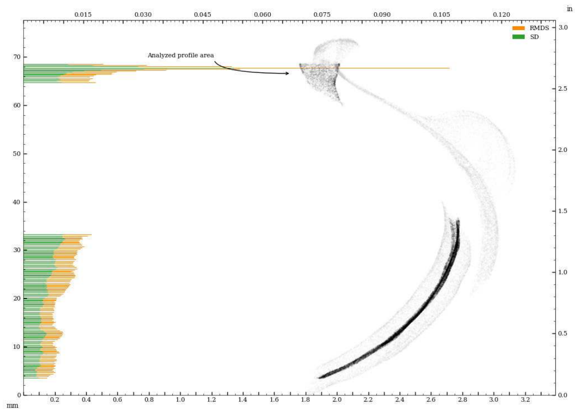
Figure 76: Vessel circularity of interior_separate surface, perpendicular to surface curvature, standard deviation and median absolute deviation.
