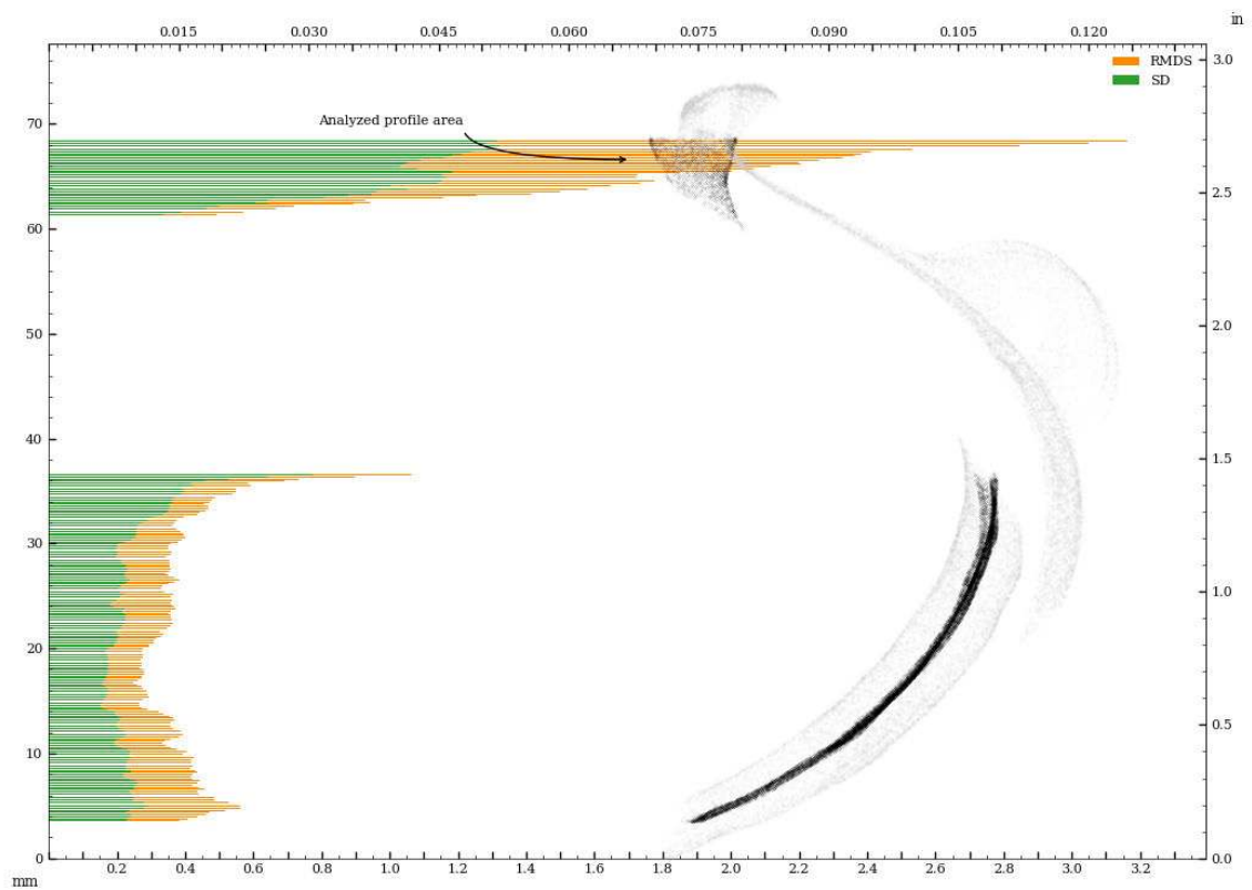
Figure 77: Vessel circularity of interior_separate surface, in z-plane, standard deviation and median absolute deviation.
