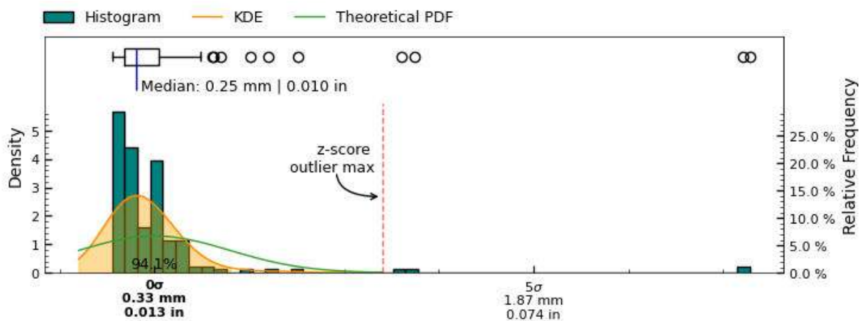
Figure 30: Root Mean Squared Deviation measurement distribution across measured slices of interior separately aligned surface
