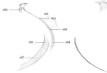
Figure 32: Circularity measurement sample locations, full mesh aligned to exterior surface
