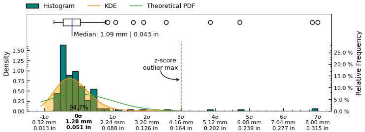
Figure 28: Range measurement distribution across measured slices of interior_separate surface
