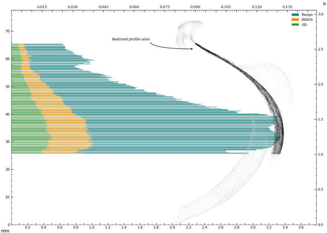
Figure 66: Circularity of exterior surface - perpendicular to surface curvature.
