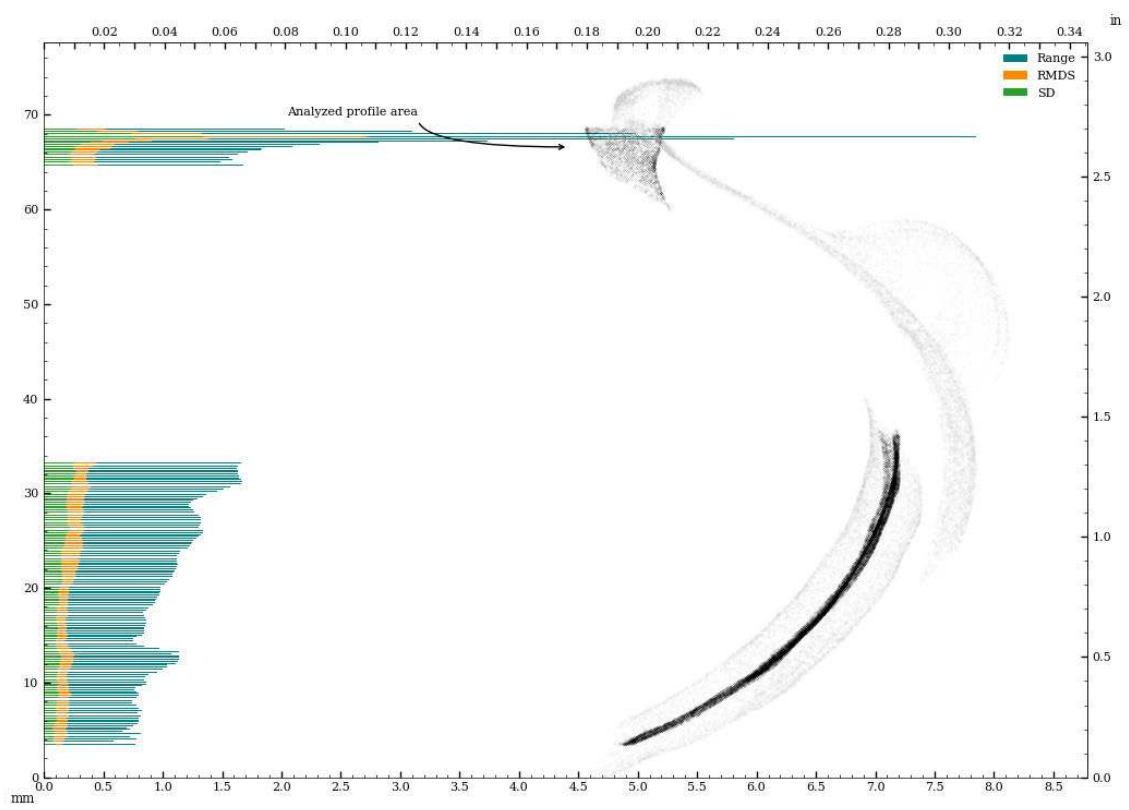
Figure 74: Circularity of interior_separate surface - perpendicular to surface curvature.
