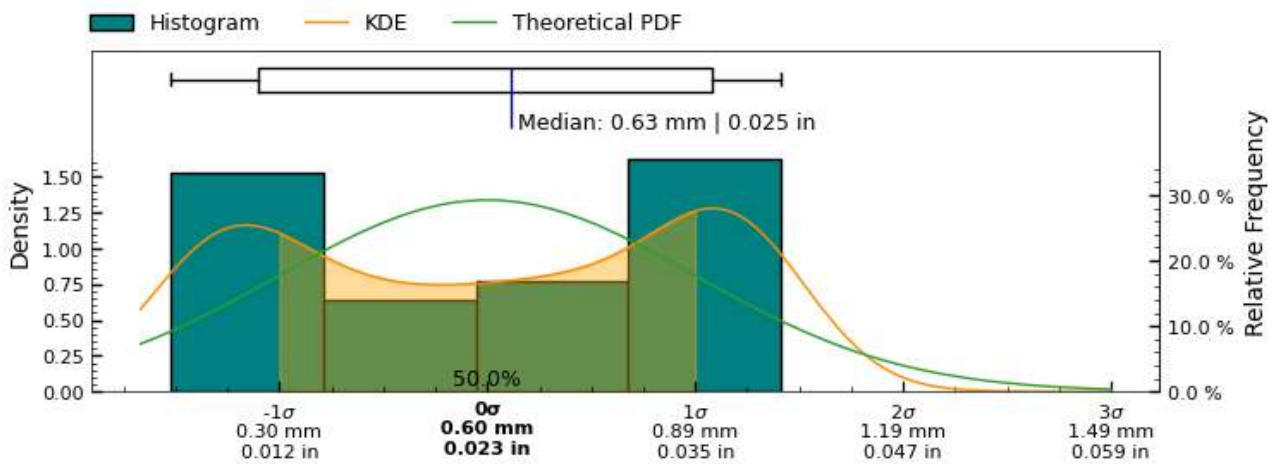
Figure 20: Root Mean Squared Deviation measurement distribution across measured slices of exterior surface
