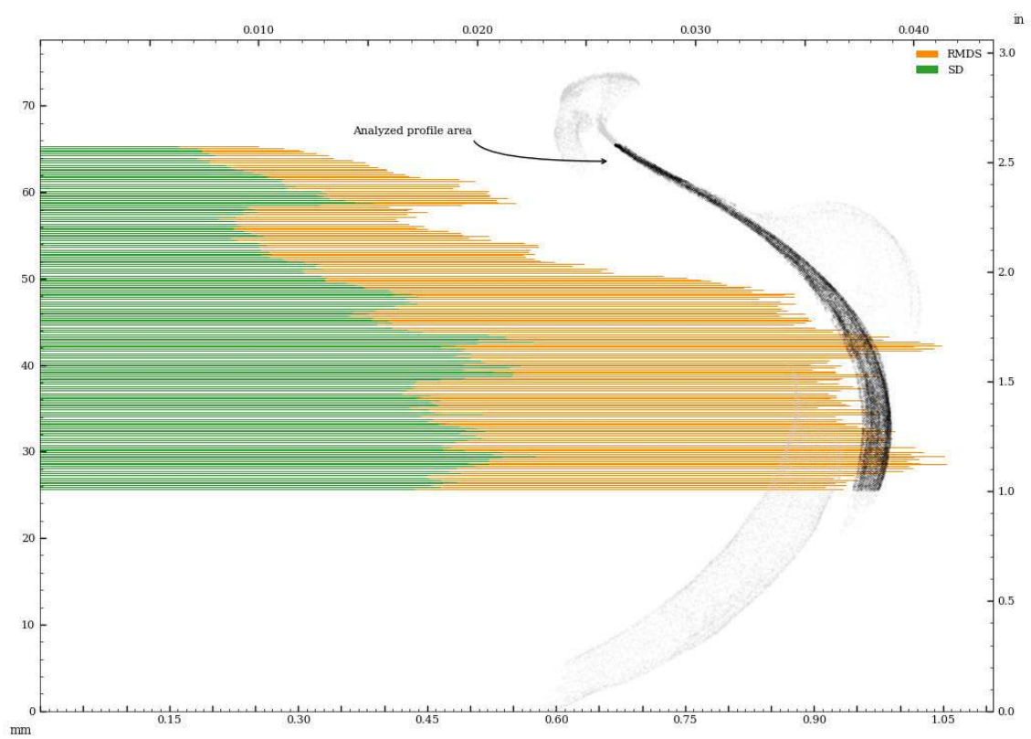
Figure 69: Vessel circularity of exterior surface, in z-plane, standard deviation and median absolute deviation.
