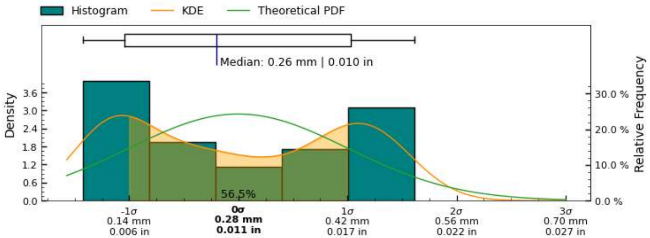
Figure 19: Standard Deviation measurement distribution across measured slices of " + exterior + " surface
