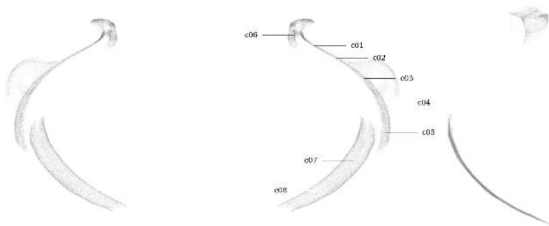
Figure 66: Circularity measurement sample locations, full mesh aligned to exterior surface
