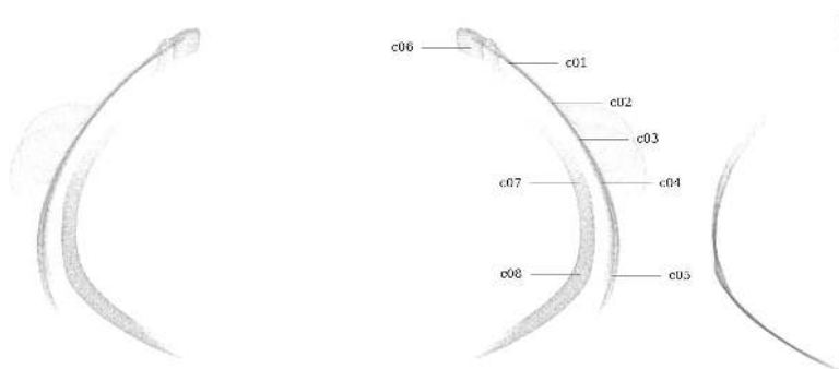
Figure 66: Circularity measurement sample locations, full mesh aligned to exterior surface
