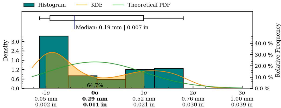
Figure 48: Coaxiality residual plots of interior_separate surface, MV025b.
