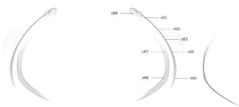
Figure 64: Circularity measurement sample locations, full mesh aligned to exterior surface
