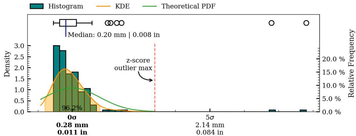
Figure 47: Coaxiality residual plots of interior surface, MV025b.
