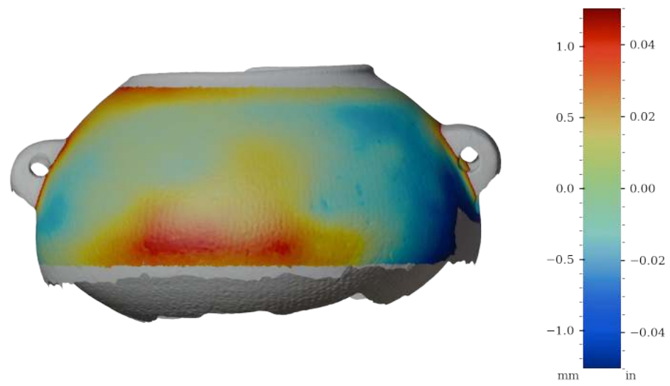
Figure 51: Surface variability heatmap of MV025b, rotated 180°
