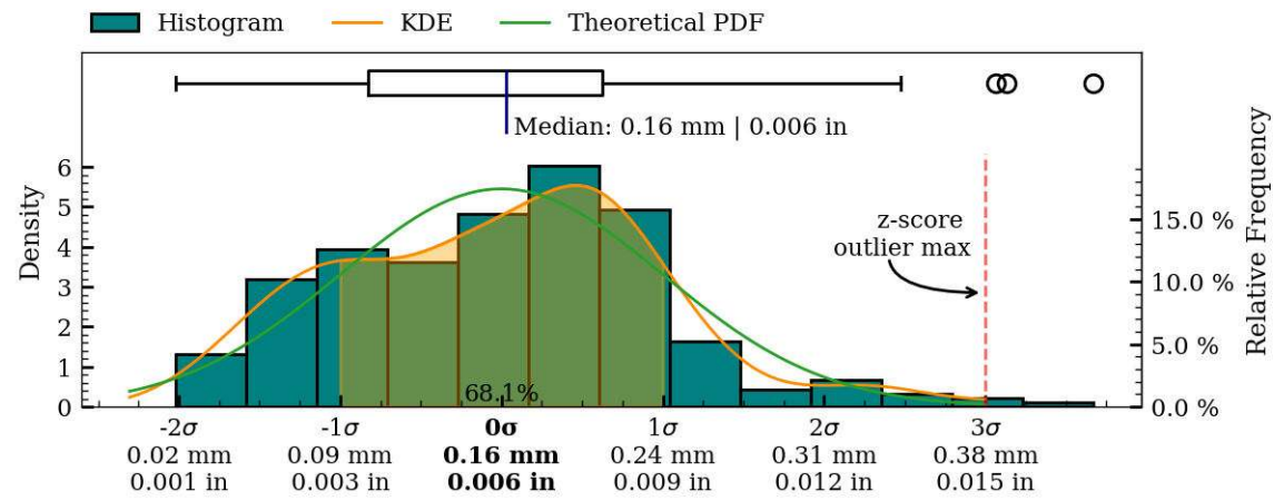
Figure 46: Coaxiality residual plots of exterior surface, MV025b.
