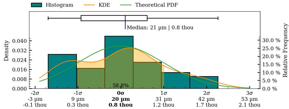
Figure 44: Coaxiality residual plots of interior_separate surface, MV026.
