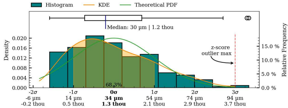
Figure 42: Coaxiality residual plots of exterior surface, MV026.
