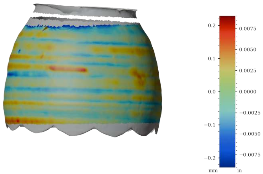
Figure 64: Surface variability heatmap of MV027, rotated 270°
