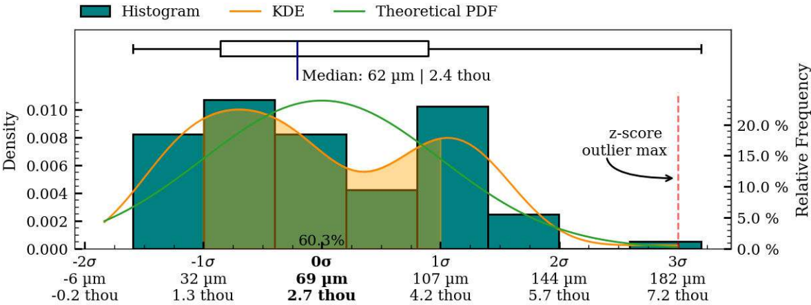
Figure 51: Coaxiality residual plots of interior surface, MV027.
