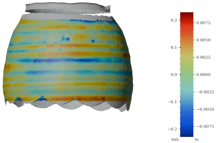
Figure 63: Surface variability heatmap of MV027, rotated 180°
