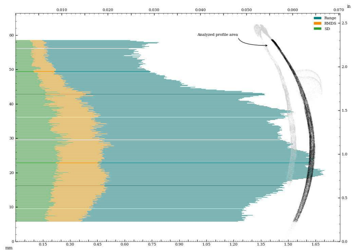
Figure 73: Circularity of exterior surface - in z-plane.
