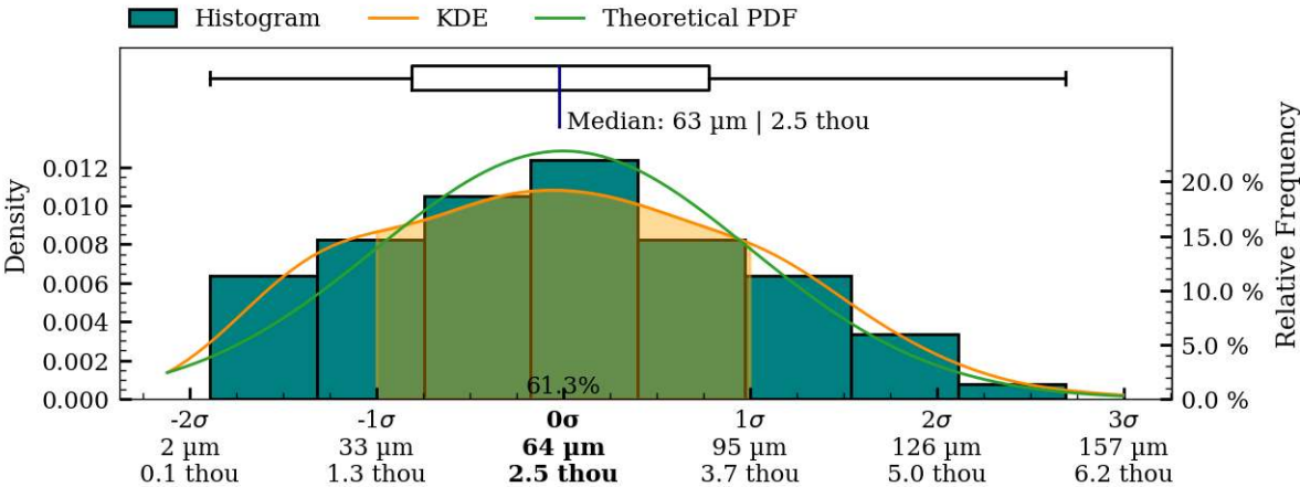
Figure 47: Coaxiality residual plots of interior surface, MV027b.
