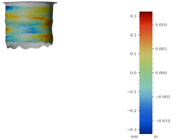
Figure 55: Surface variability heatmap of MV030, rotated 180°
