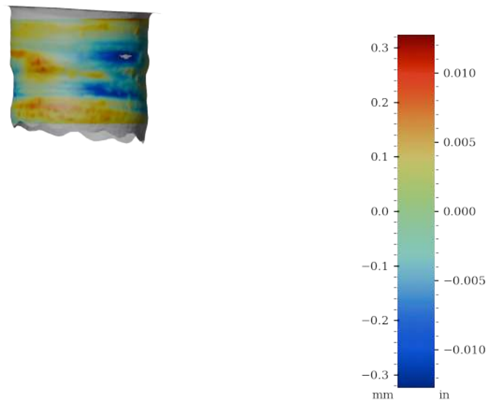
Figure 56: Surface variability heatmap of MV030, rotated 270°
