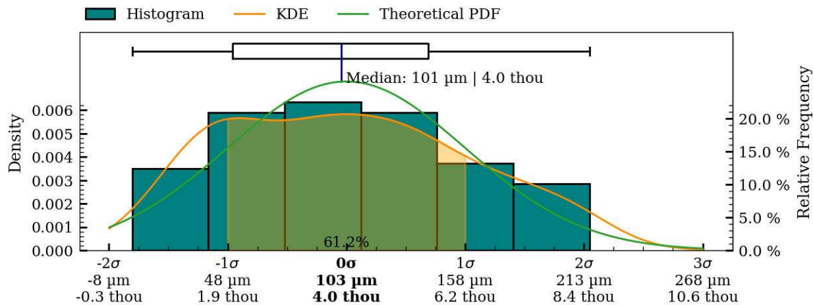
Figure 44: Coaxiality residual plots of interior_separate surface, MV030.
