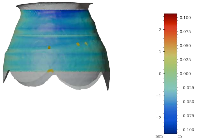
Figure 52: Surface variability heatmap of MV032, rotated 270°
