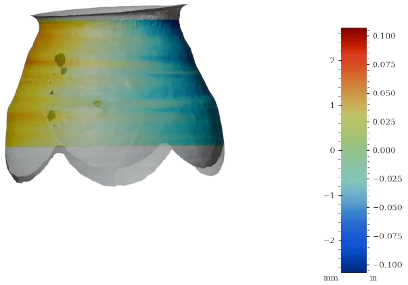
Figure 51: Surface variability heatmap of MV032, rotated 180°
