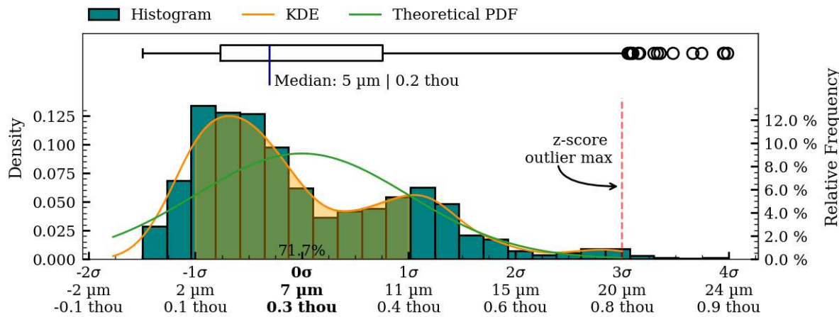
Figure 44: Coaxiality residual plots of exterior surface, PV001.
