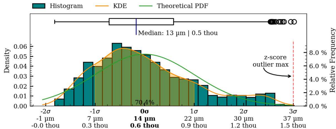
Figure 45: Coaxiality residual plots of interior surface, PV001.
