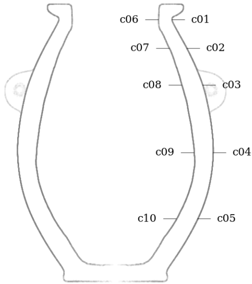
Figure 64: Circularity measurement sample locations, full mesh aligned to exterior surface
