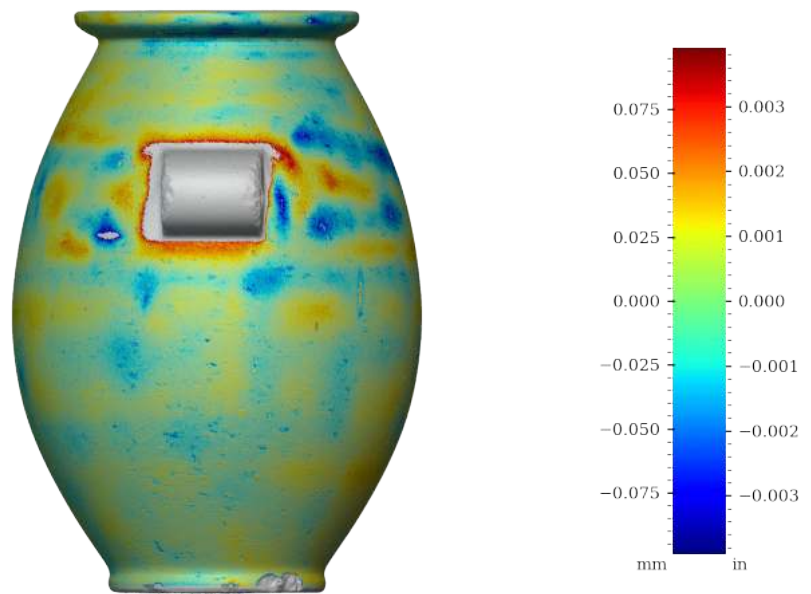
Figure 50: Surface variability heatmap of PV001, rotated 270°
