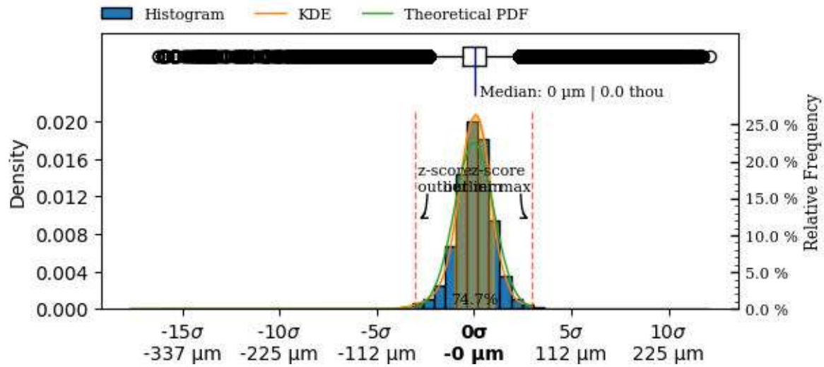
Figure 59: Exterior surface variability boxplot, kds and histogram.
