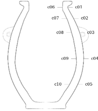
Figure 32: Circularity measurement sample locations, full mesh aligned to exterior surface
