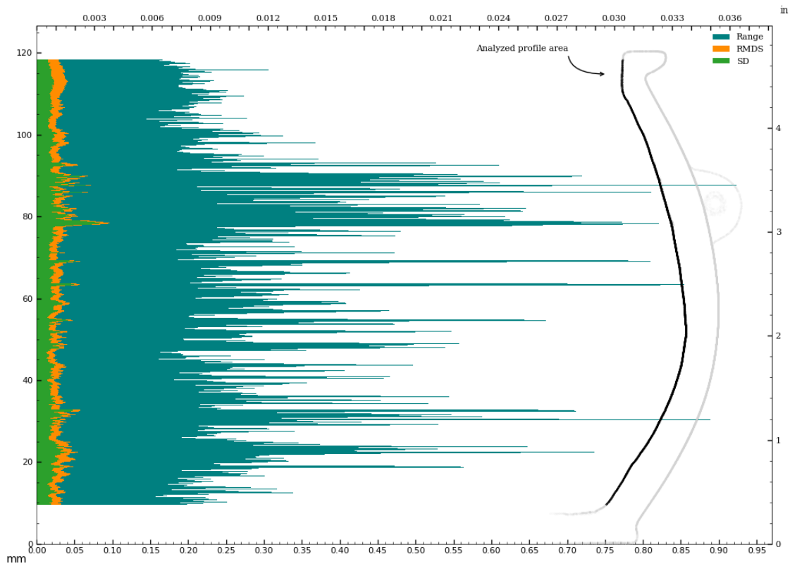
Figure 75: Circularity of interior_separate surface - in z-plane.
