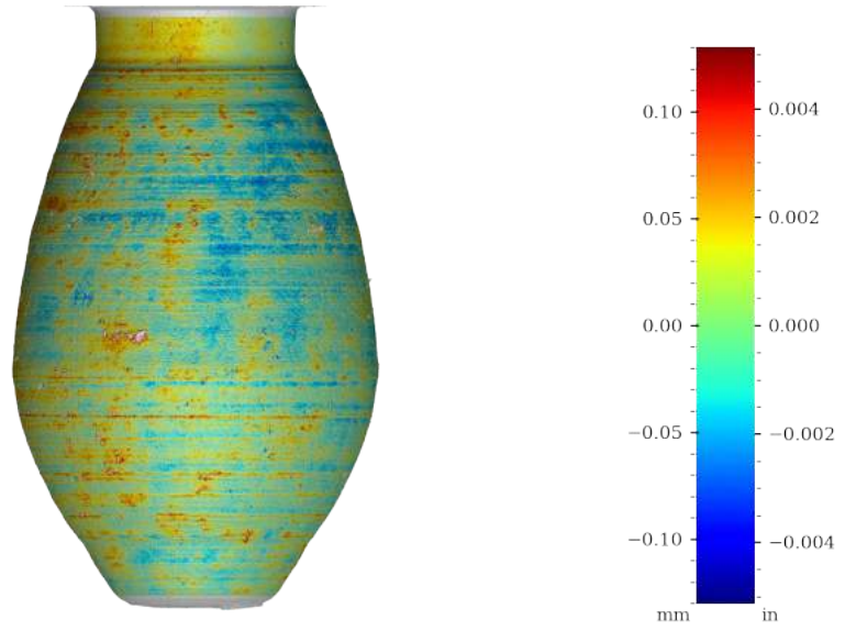
Figure 53: Surface variability heatmap of PV001, rotated 180°
