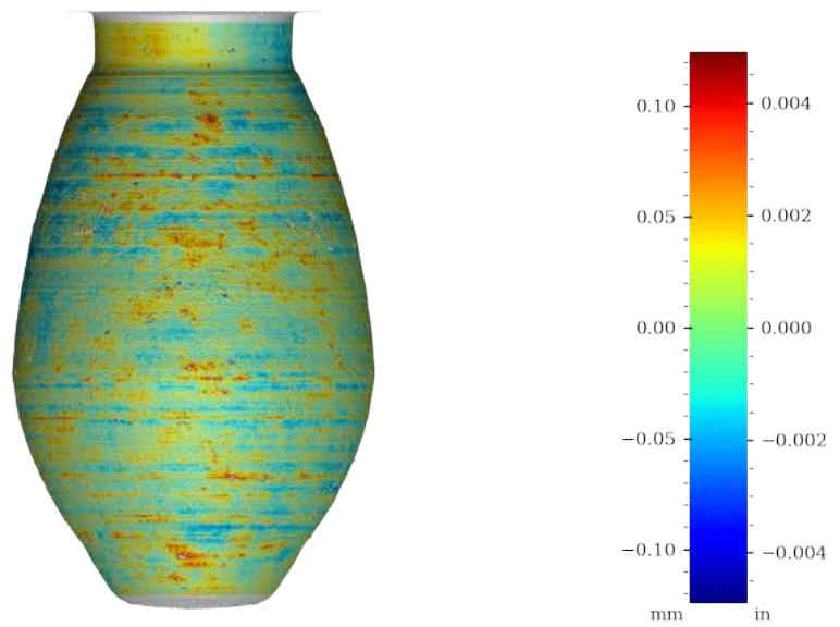
Figure 58: Surface variability heatmap of PV001, rotated 270°
