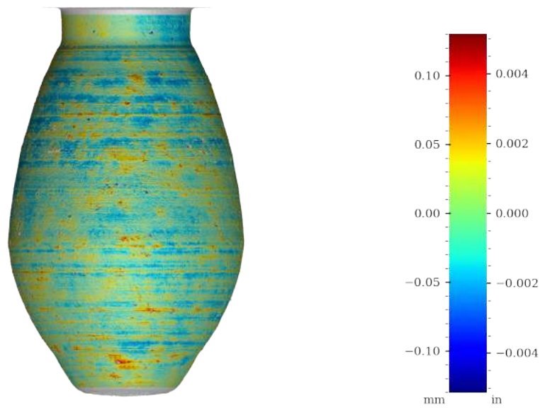
Figure 54: Surface variability heatmap of PV001, rotated 270°
