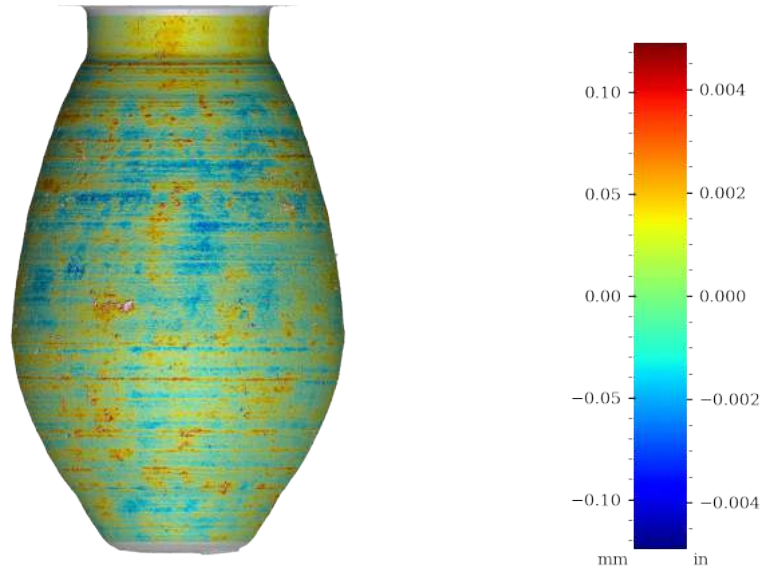
Figure 57: Surface variability heatmap of PV001, rotated 180°
