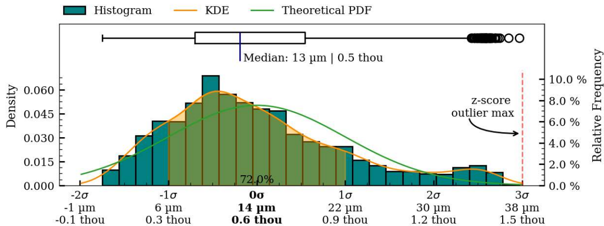
Figure 46: Coaxiality residual plots of interior_separate surface, PV001.
