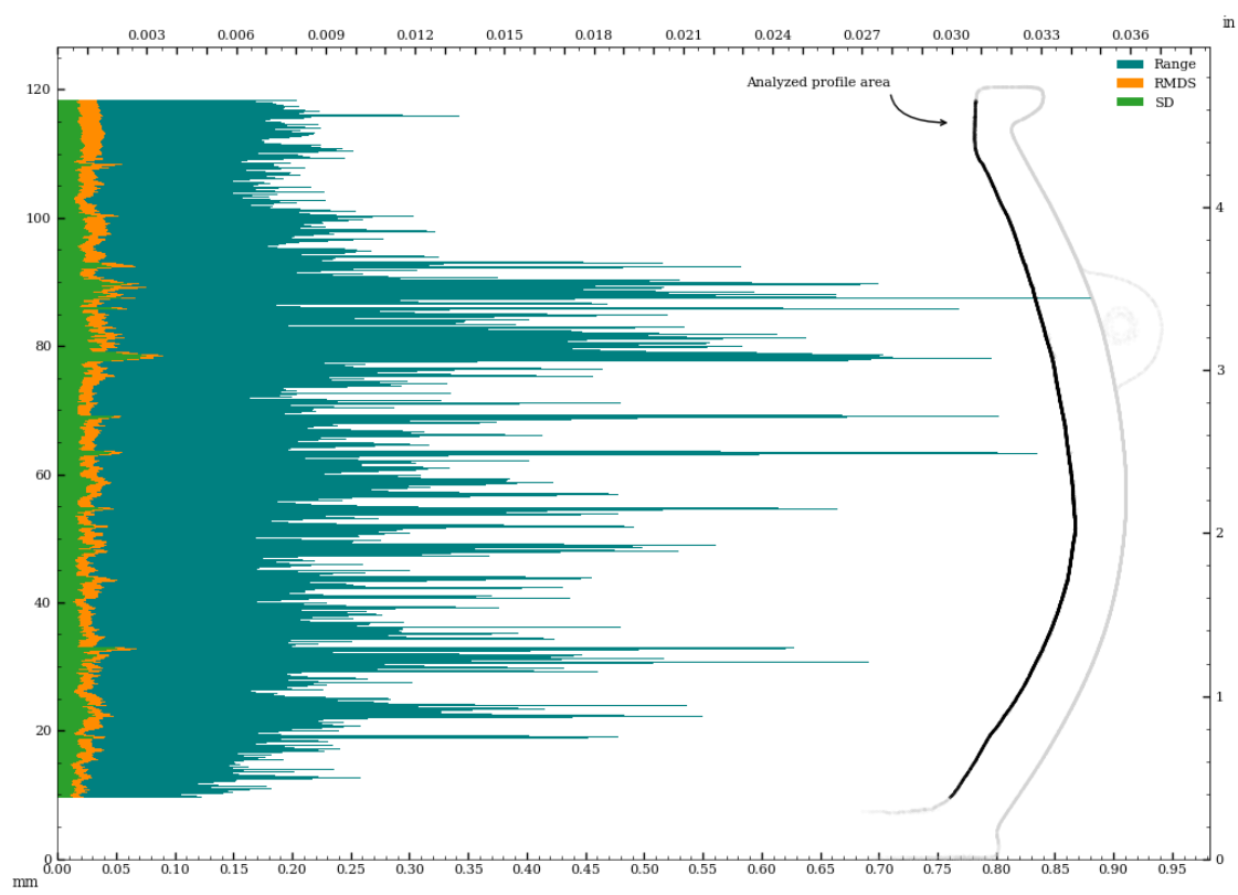
Figure 70: Circularity of interior surface - perpendicular to surface curvature.
