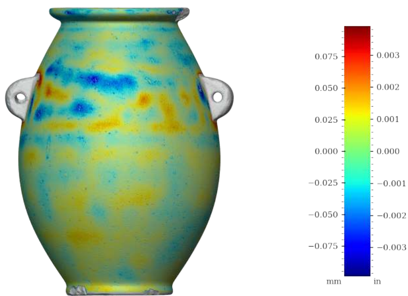
Figure 47: Surface variability heatmap of PV001, front view
