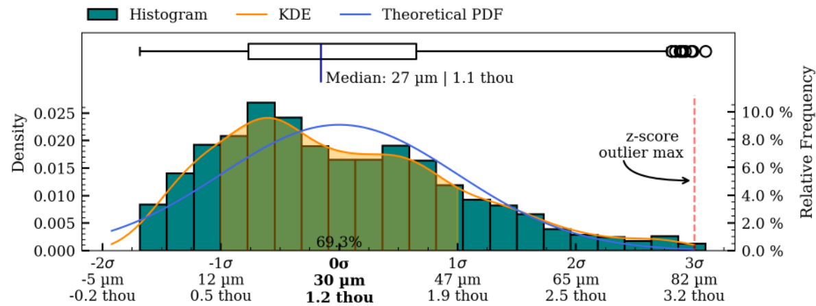
Figure 56: Coaxiality residual plots of interior_separate surface, PV003.
