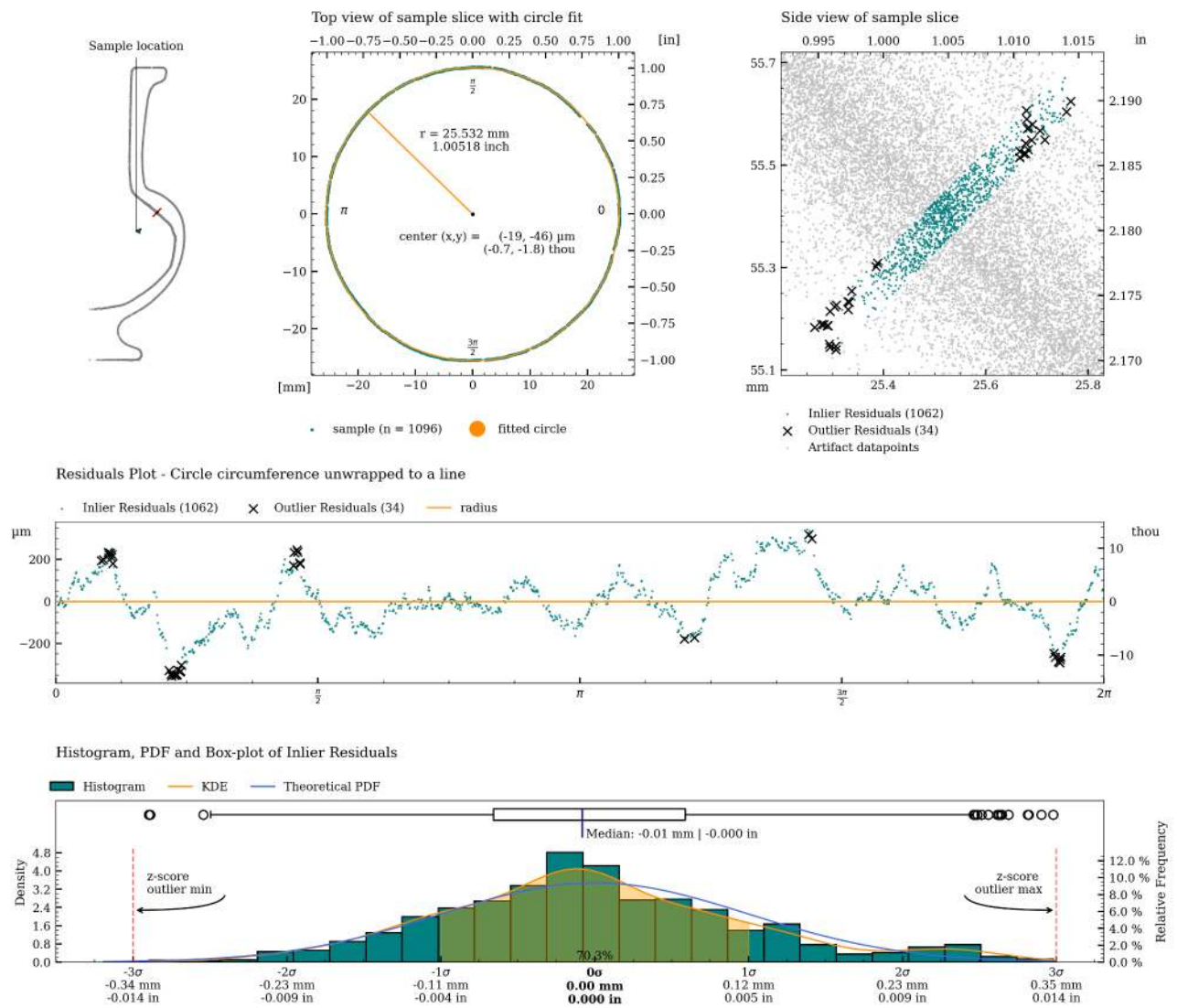
Figure 48: Detailed plot of concentricity measurement for c08.
