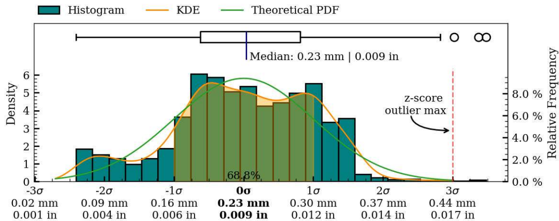
Figure 52: Coaxiality residual plots of interior_separate surface, RV001.
