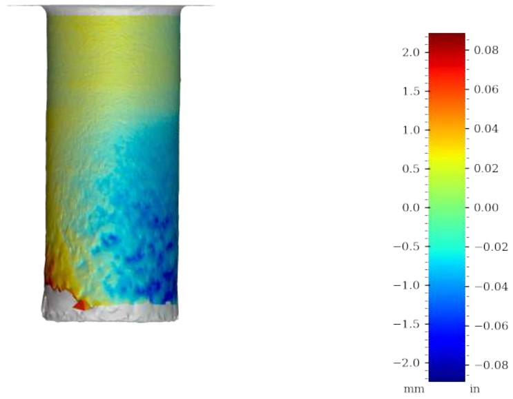
Figure 59: Surface variability heatmap of RV001, rotated 180°
