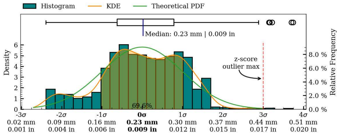
Figure 51: Coaxiality residual plots of interior surface, RV001.
