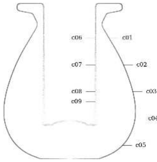
Figure 68: Circularity measurement sample locations, full mesh aligned to exterior surface
