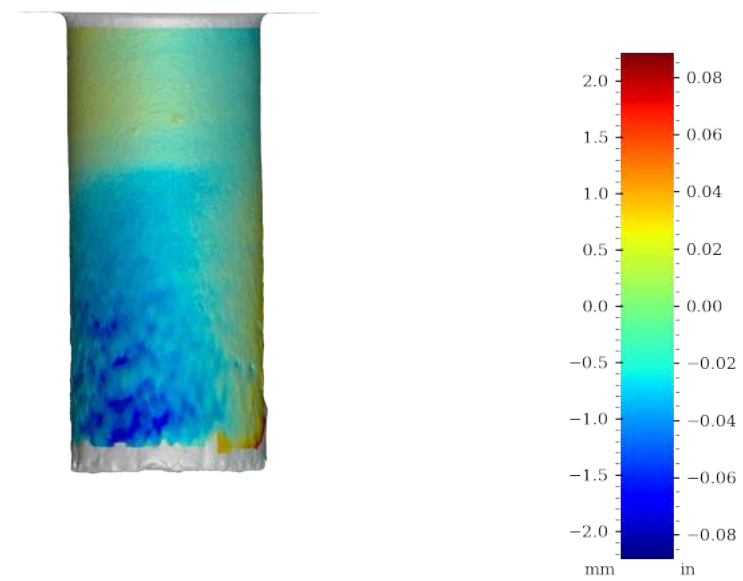
Figure 60: Surface variability heatmap of RV001, rotated 270°
