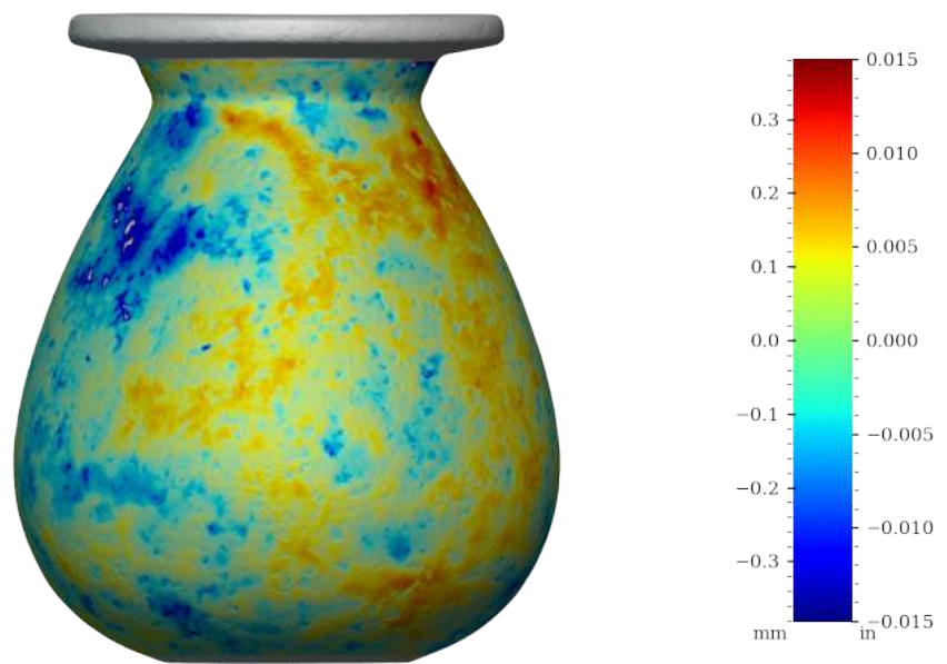
Figure 56: Surface variability heatmap of RV001, rotated 270°
