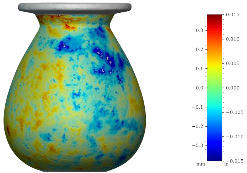
Figure 55: Surface variability heatmap of RV001, rotated 180°
