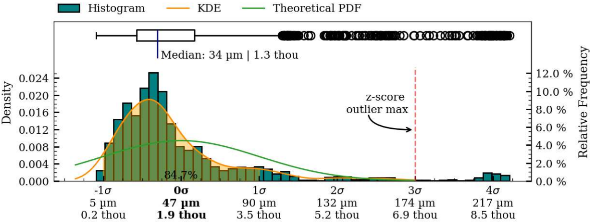
Figure 50: Coaxiality residual plots of exterior surface, RV001.
