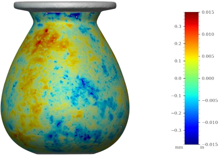
Figure 53: Surface variability heatmap of RV001, front view
