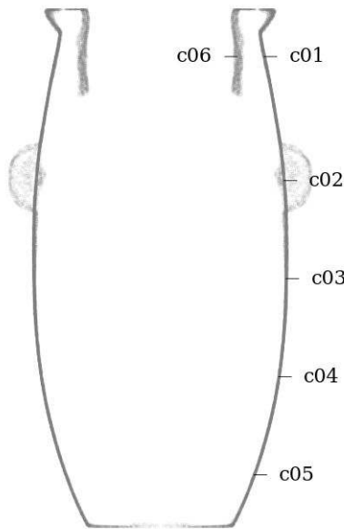
Figure 72: Circularity measurement sample locations, full mesh aligned to exterior surface
