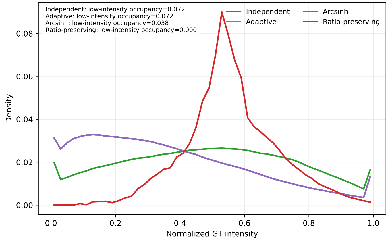
Normalization Strategy Comparison (GT Histogram)
