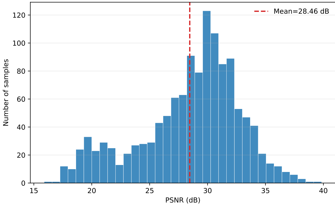
Per-sample PSNR Distribution (exp009, N=1272)
