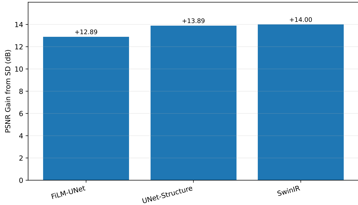
Same-Backbone SD Ablation (N=1272)
