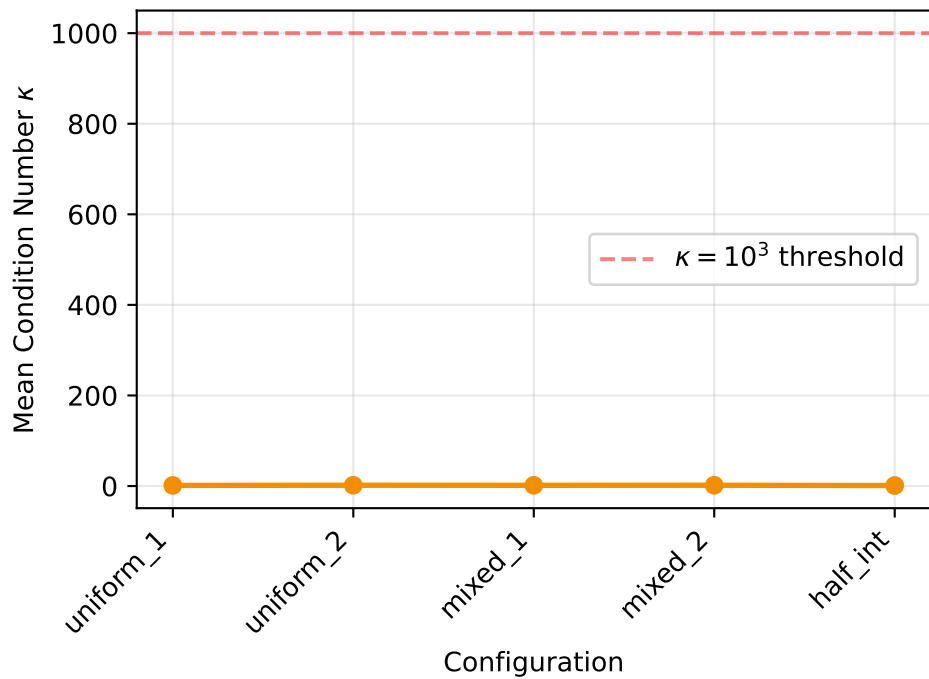
Recurrence Condition Numbers
