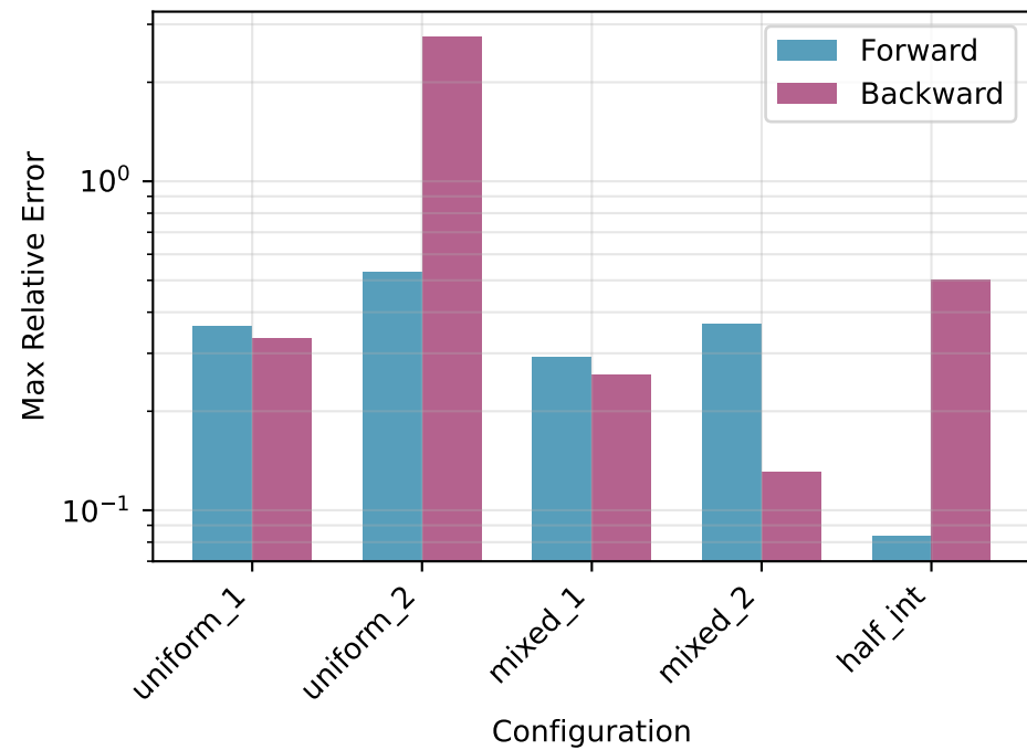
Recurrence Error: Forward vs Backward
