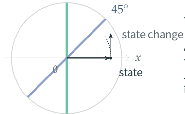
Bloch-plane view
