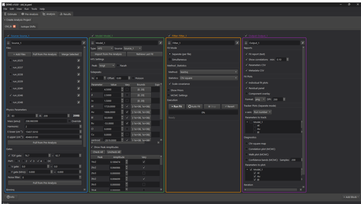
Figure 6: An Analysis project (here, an 209 Bi fit) showing the four-block pipeline from left to right: Source (file selection, physics parameters, ToF and binning), Model (HFS settings, parameter table with per-parameter modes, peak amplitudes), Fitter (method, statistics, execution controls), and Output (which reports, plots, and diagnostics to produce).
