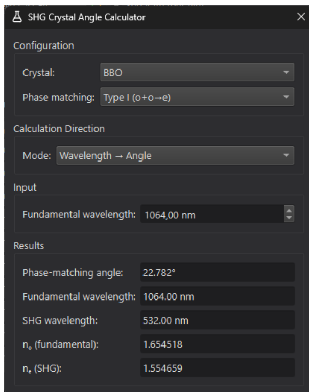
Figure 11: SHG Crystal Angle Calculator: BBO Type-I phase-matching angle ( 22.78^\circ ) for the second harmonic of 1064 nm.
