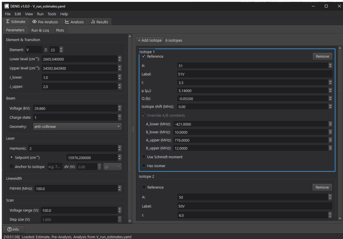
Figure 3: Estimate tab with the global parameters ( Element & Transition , Beam , Laser , Linewidth , Scan ) filled in for a vanadium chain, and the first isotope panel ( ^{51}\text{V} , marked Reference ) expanded to show the per-isotope inputs and an explicit A/B override.
