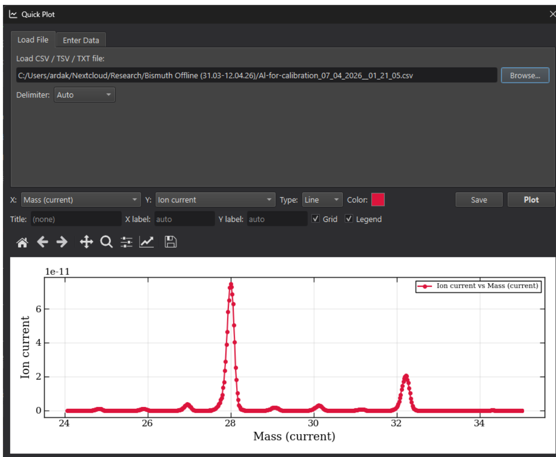
Figure 12: Quick Plot showing an ion-source mass-scan calibration loaded from CSV: ion current as a function of mass setting, with the sample isotopes appearing as well-resolved peaks near A = 28 and A = 32 .
