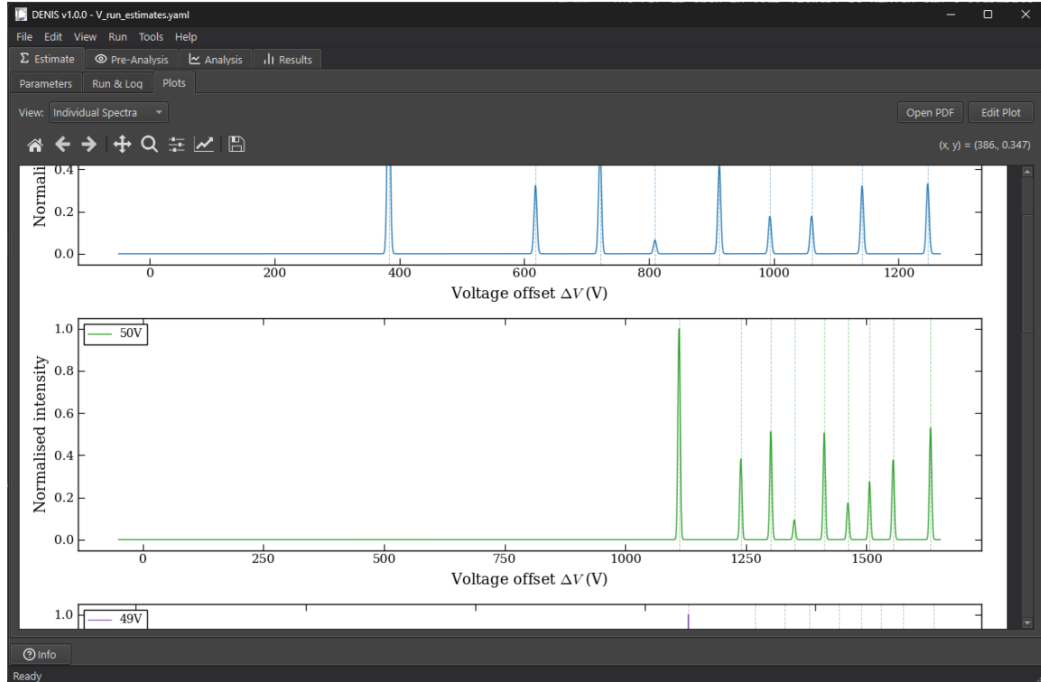
(b) The plot panel. Each isotope gets its own simulated voltage spectrum on the requested scan range; dashed lines mark the individual hyperfine peaks.
