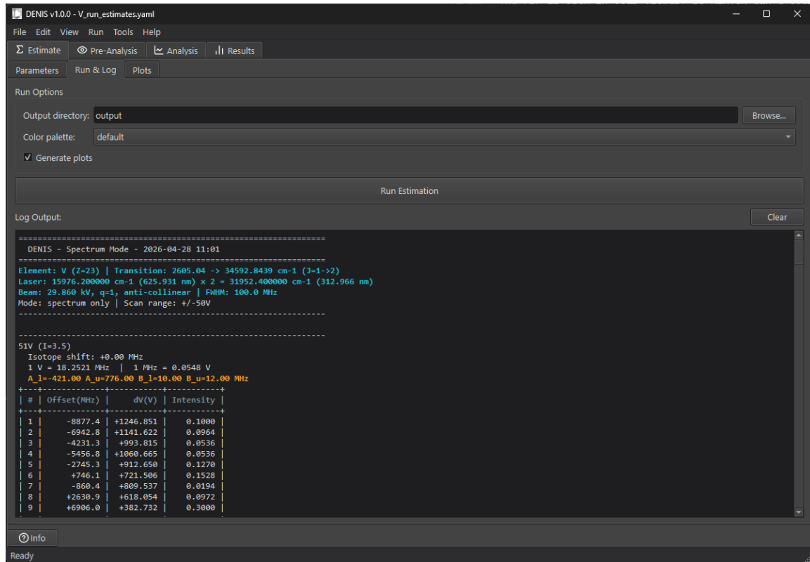
(a) The run log. The header summarises the inputs; the body lists each hyperfine peak with offset, voltage, and intensity.
