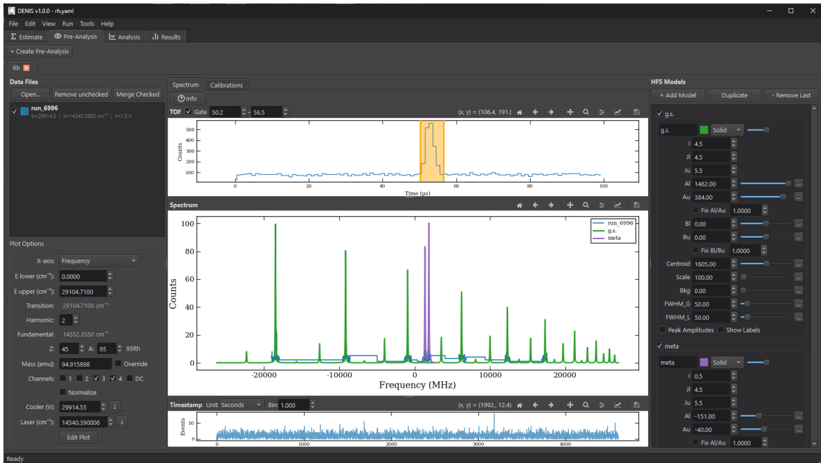
Figure 5: Pre-Analysis tab with one rhodium run loaded. Top centre: the time-of-flight spectrum with the gate highlighted in orange. Centre: the binned spectrum (blue data) with two HFS models overlaid (green ground state, purple isomer) on the right-panel parameters. Left: file list and binning controls; right: the HFS model parameter editor.
