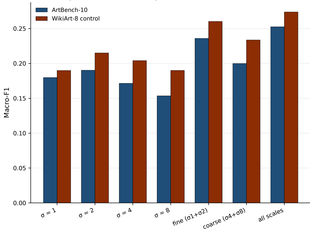
Artist-disjoint classification by spatial scale
