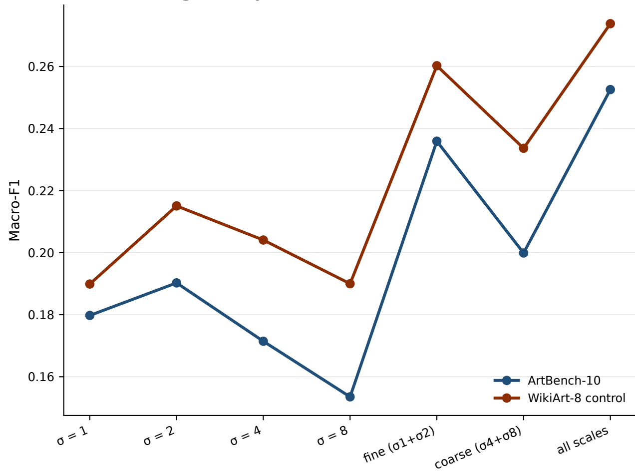
Intermediate geometry is most discriminative
