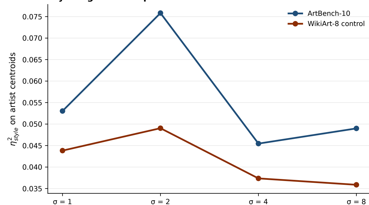
Style organisation peaks at intermediate scale
