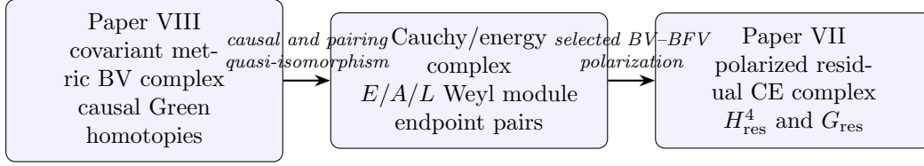
Figure 3: The VII–VIII relation. Paper VII computes the right-hand cohomology. Paper VIII proves that the covariant left-hand complex transports to it; the arrow does not conceal a second CE calculation.
