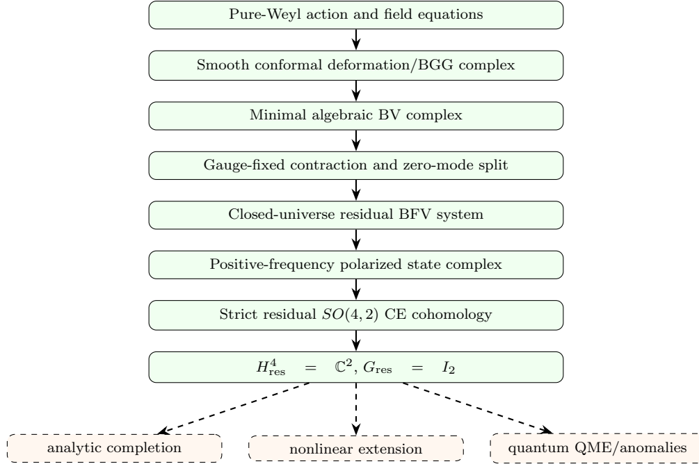
Figure 3: Completed classical theorem chain for the pure-Weyl branch. Solid arrows are proved in the stated smooth or algebraic categories; dashed arrows mark the three remaining frontiers.
