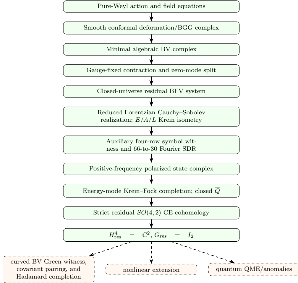
Figure 3: Completed classical theorem chain for the pure-Weyl branch. Solid arrows are proved in the stated smooth, algebraic, or energy-mode categories; dashed arrows mark the three remaining frontiers.
