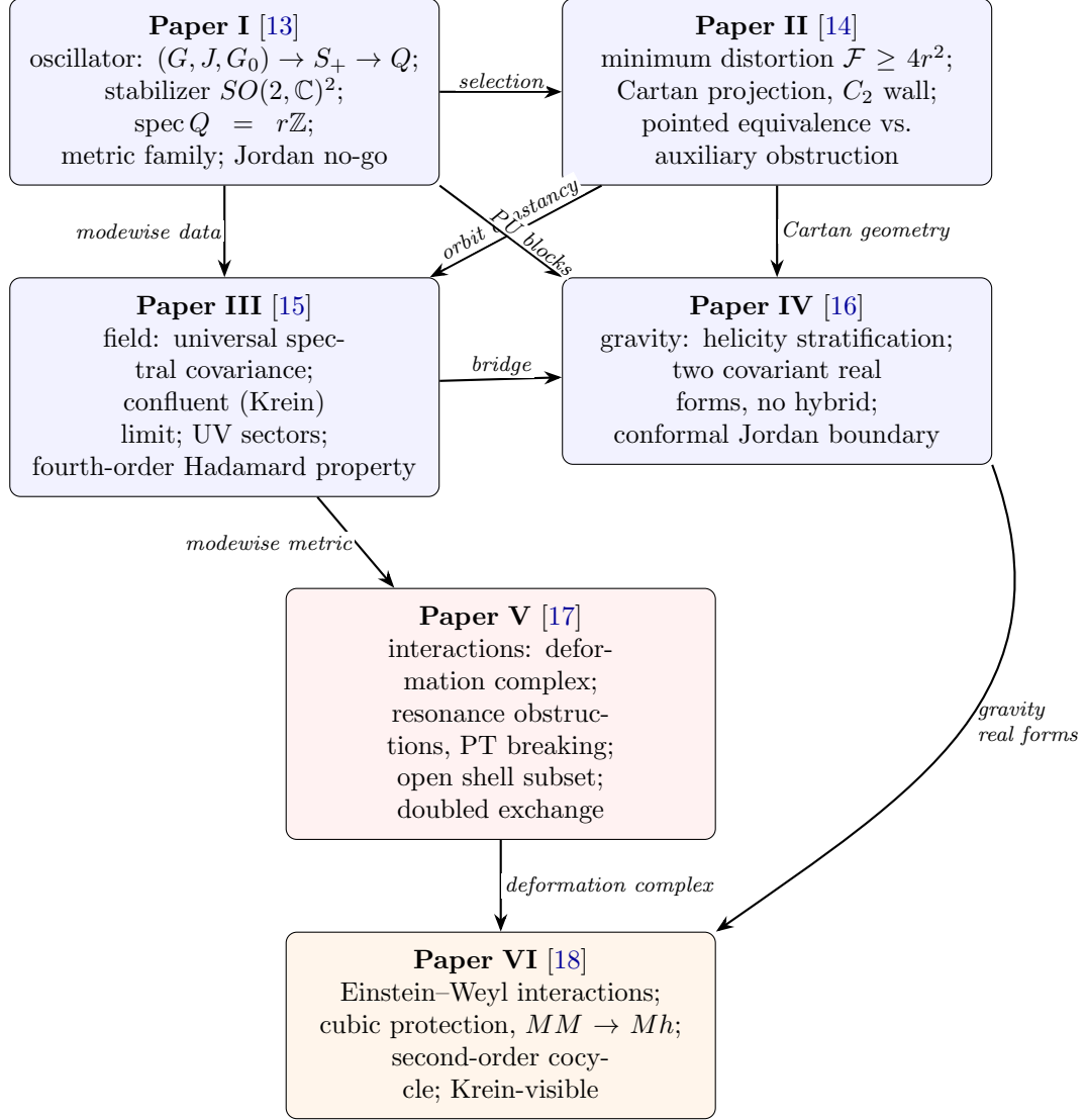
Figure 3: Dependency structure of the six technical papers. Papers I–III establish the oscillator and scalar geometry, Paper IV classifies the covariant free gravity completions, Paper V develops the interaction-obstruction framework, and Paper VI applies that framework to the Einstein–Weyl interaction.
