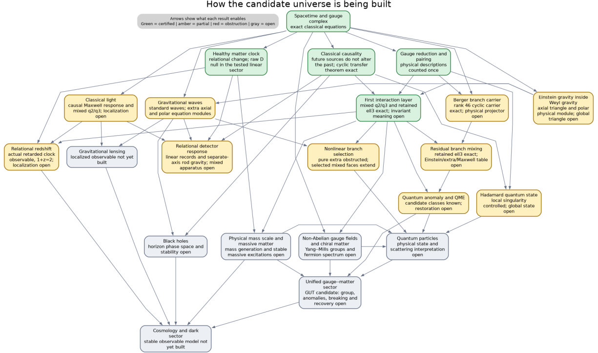
Figure 1: Certificate-backed construction map for the candidate universe
